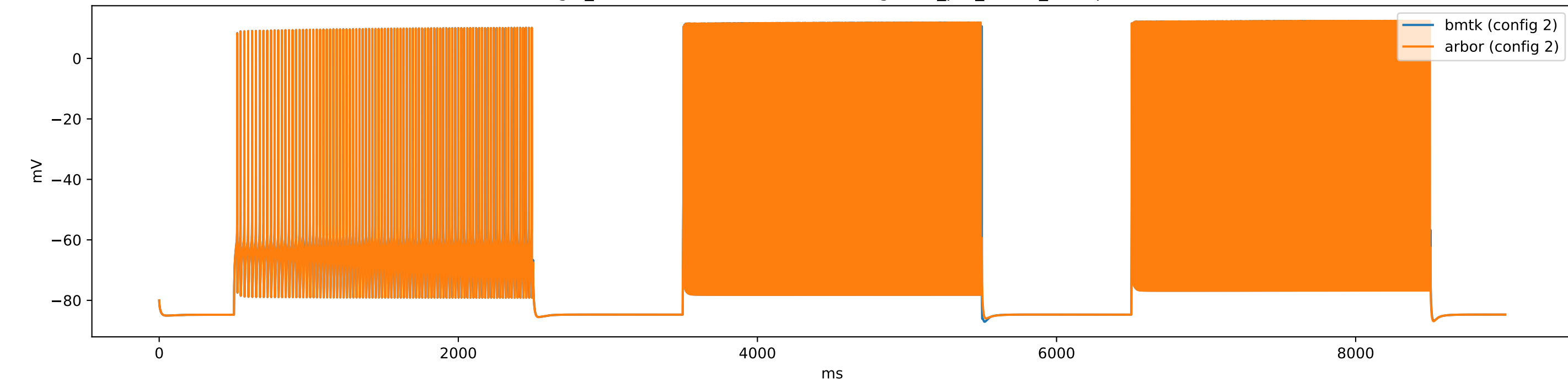
gid_108-478058328 (i6Pvalb) - config.1cell_per_model_iclamp
