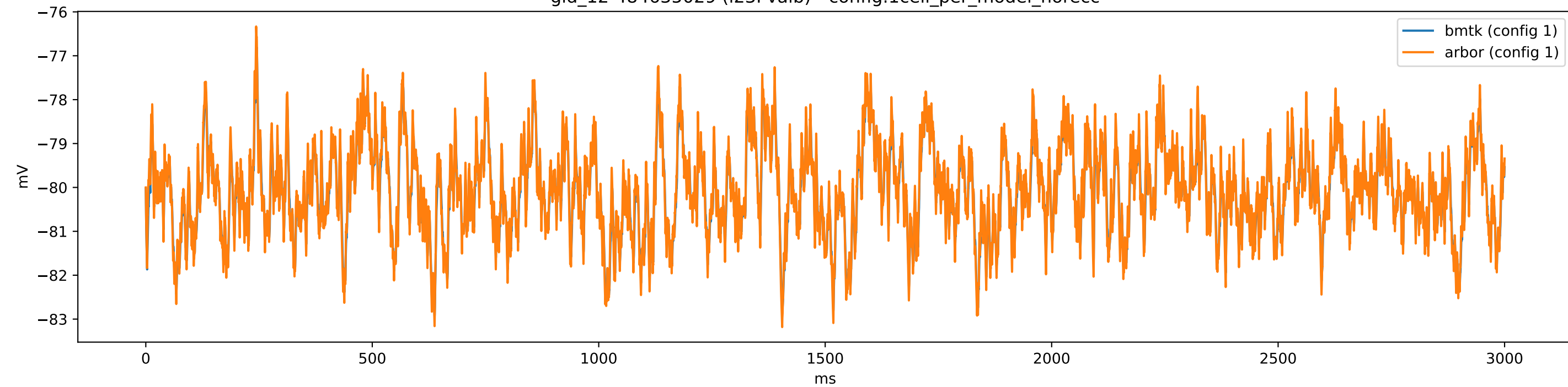
gid_12-484635029 (i23Pvalb) - config.1cell_per_model_iclamp
