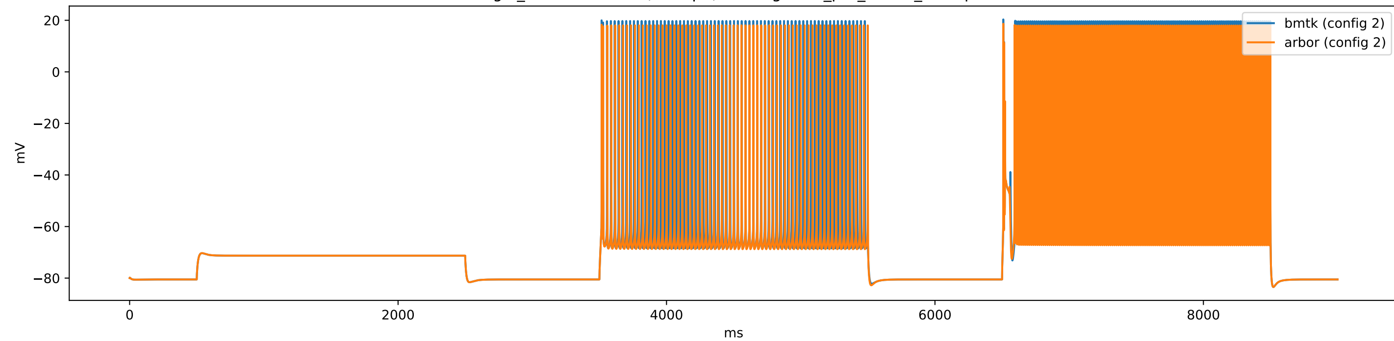
gid_61-486052980 (e5Rbp4) - config.1cell_per_model_iclamp
