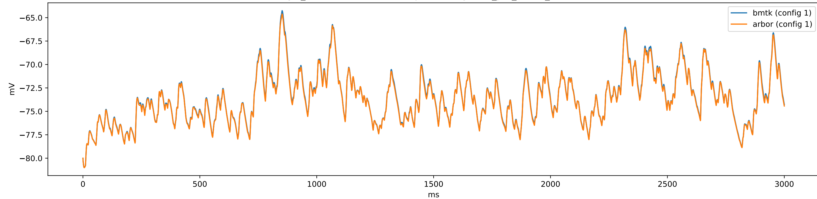
gid_65-314831019 (e5noRbp4) - config.1cell_per_model_iclamp
