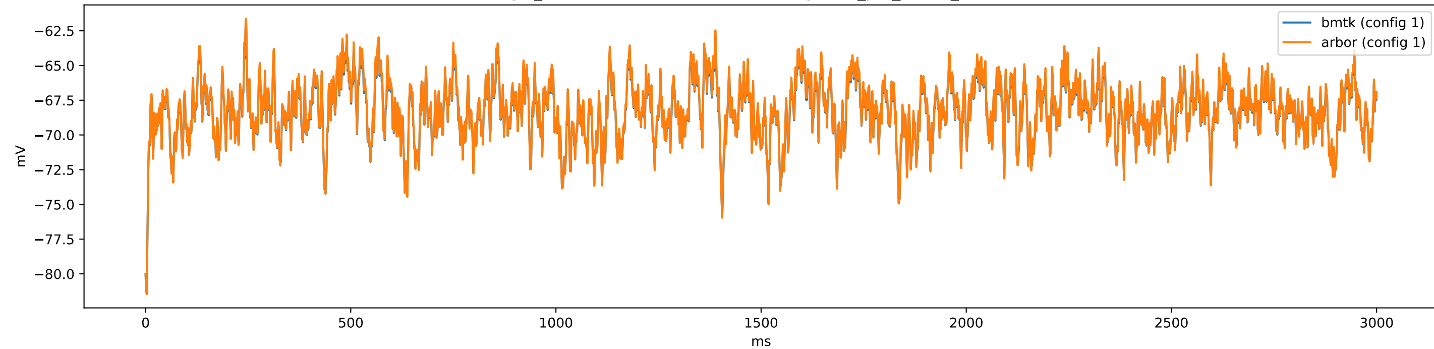
gid_10-479220013 (i23Htr3a) - config.1cell_per_model_iclamp
