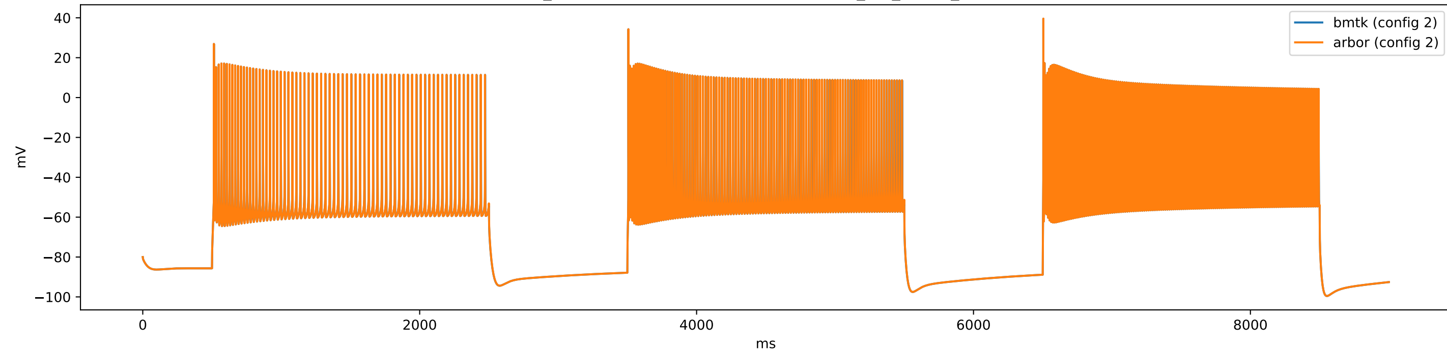
gid_37-486502127 (e4Rorb) - config.1cell_per_model_iclamp
