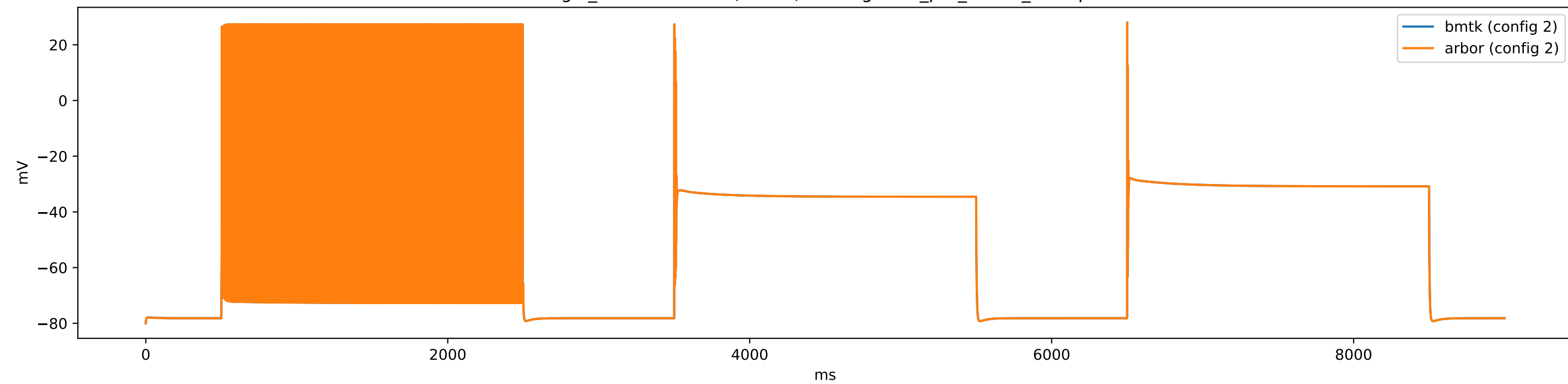
gid_17-476686112 (i23Sst) - config.1cell_per_model_iclamp
