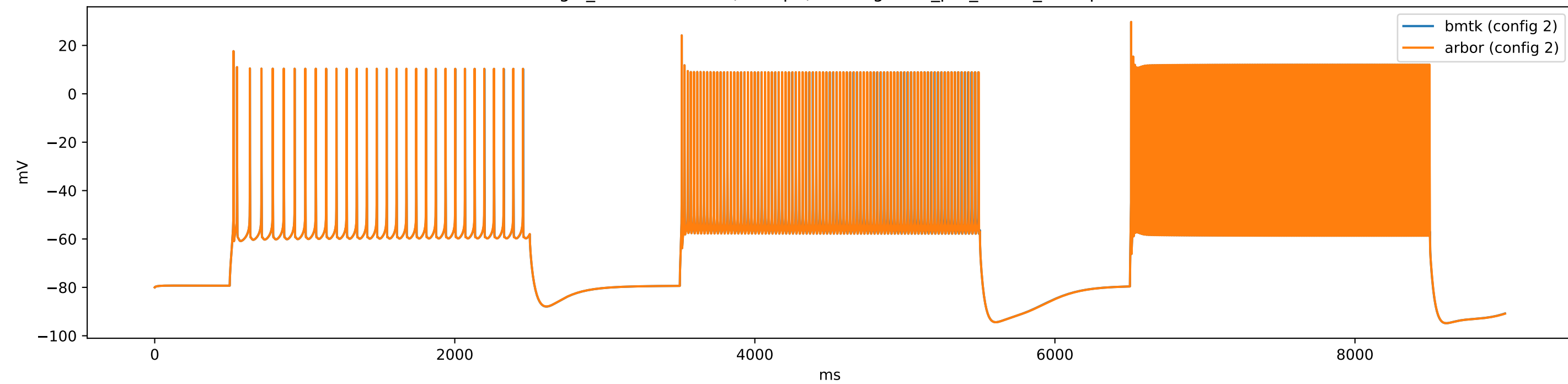
gid_63-487664663 (e5Rbp4) - config.1cell_per_model_iclamp
