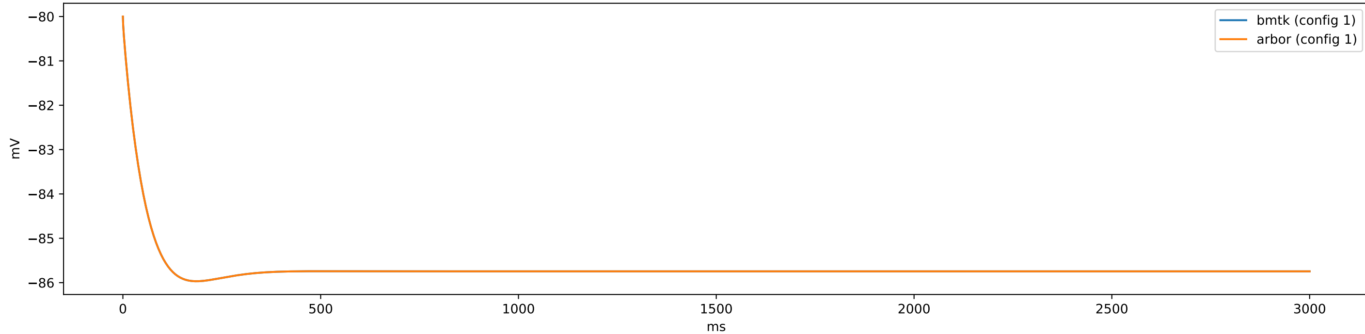
gid_104-581001895 (i6Htr3a) - config.1cell_per_model_iclamp
