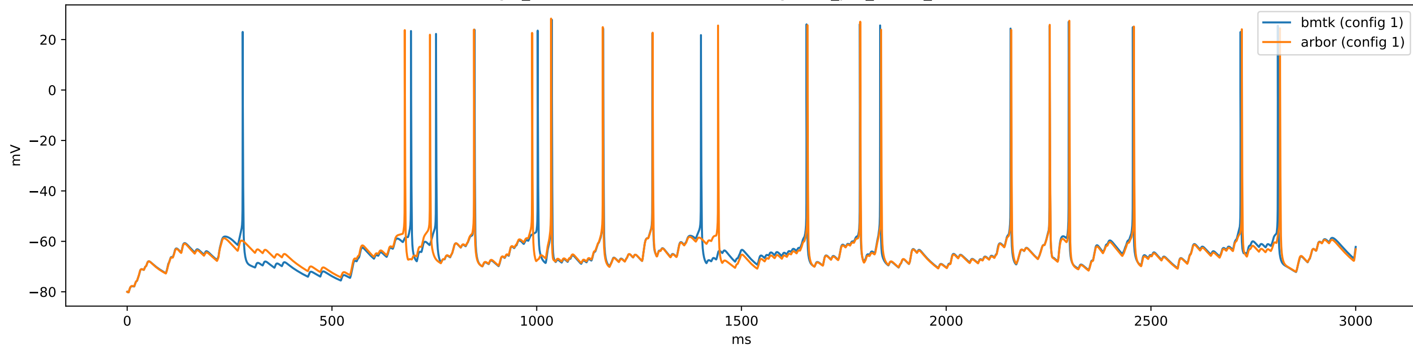
gid_33-480087928 (e4Rorb) - config.1cell_per_model_iclamp
