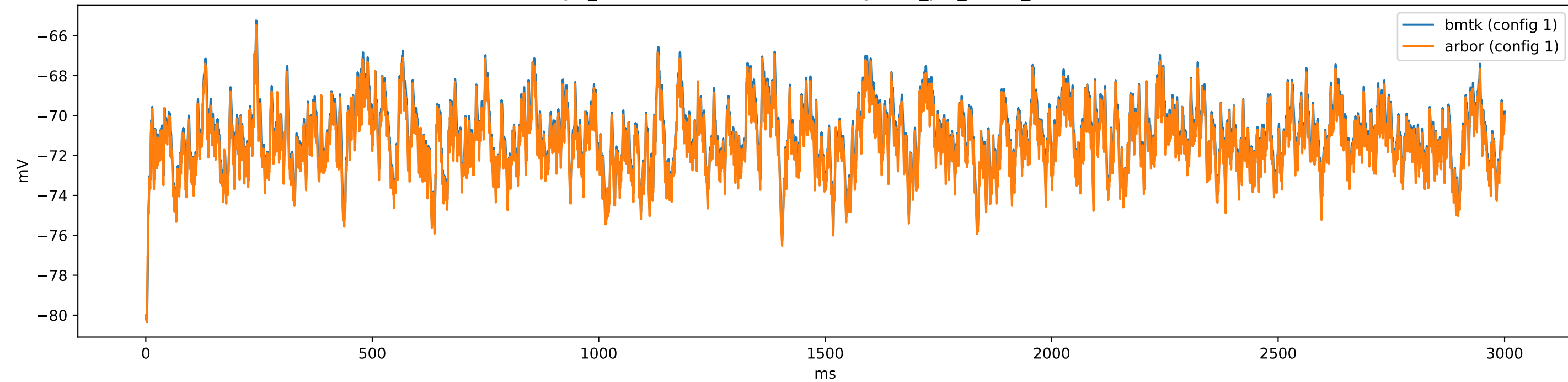
gid_16-475068599 (i23Sst) - config.1cell_per_model_iclamp
