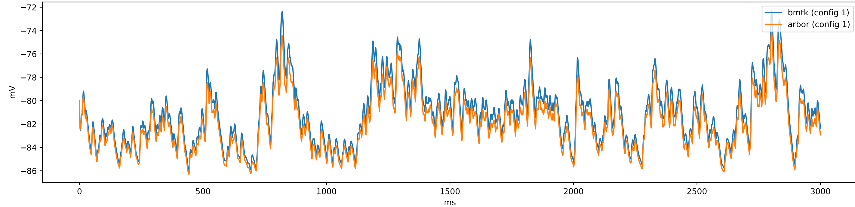
gid_101-471786879 (e6Ntsr1) - config.1cell_per_model_iclamp
