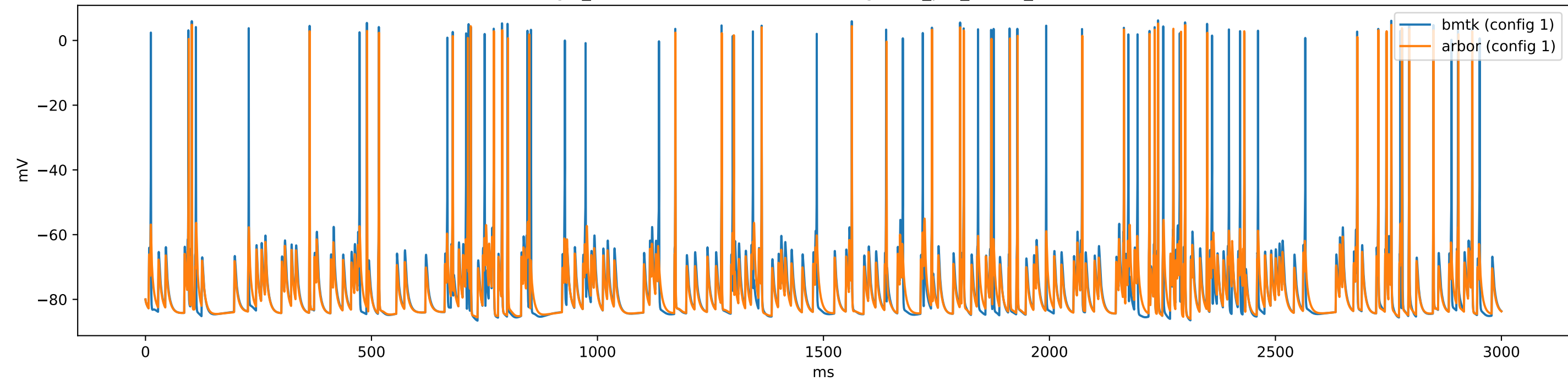
gid_88-396608557 (i5Pvalb) - config.1cell_per_model_iclamp
