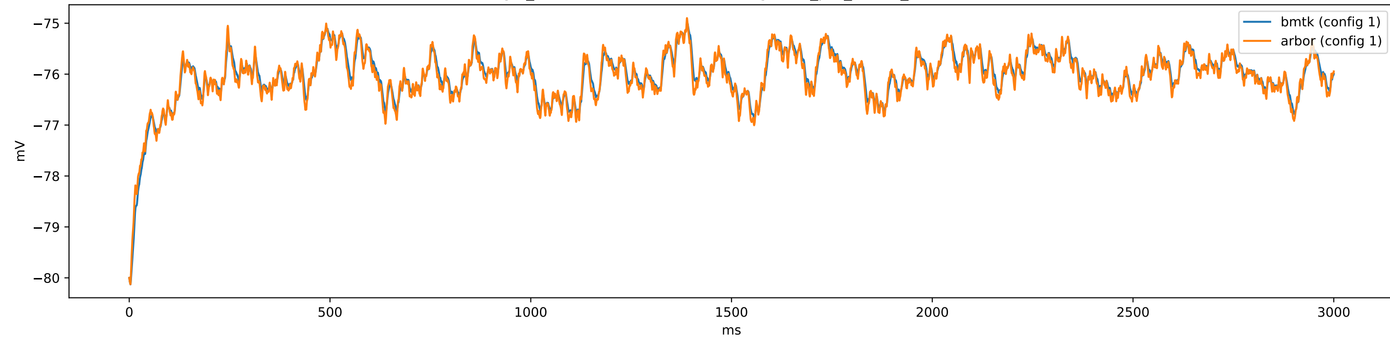
gid_97-478396248 (i5Sst) - config.1cell_per_model_iclamp
