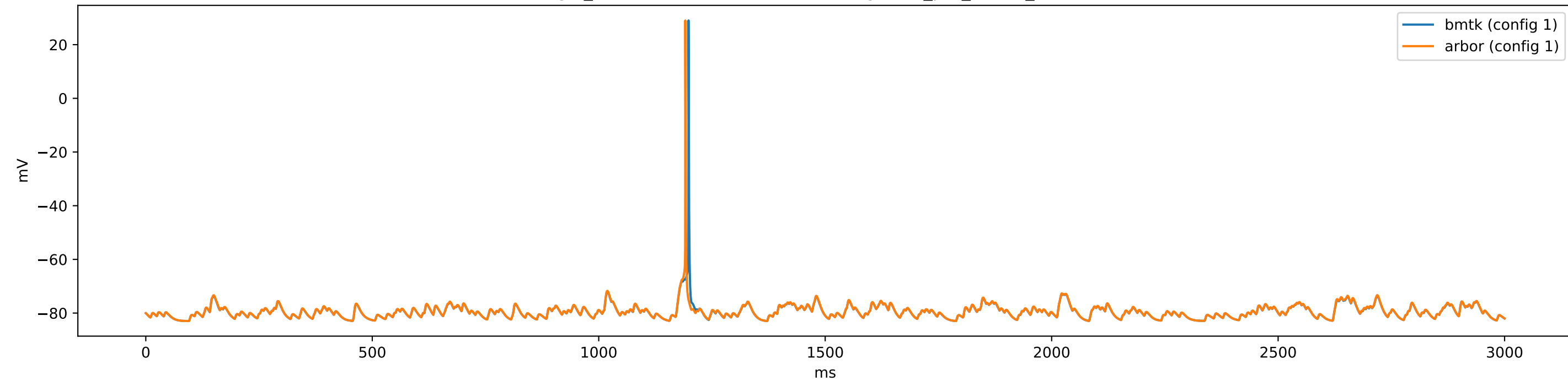
gid_31-476616076 (e4Rorb) - config.1cell_per_model_iclamp
