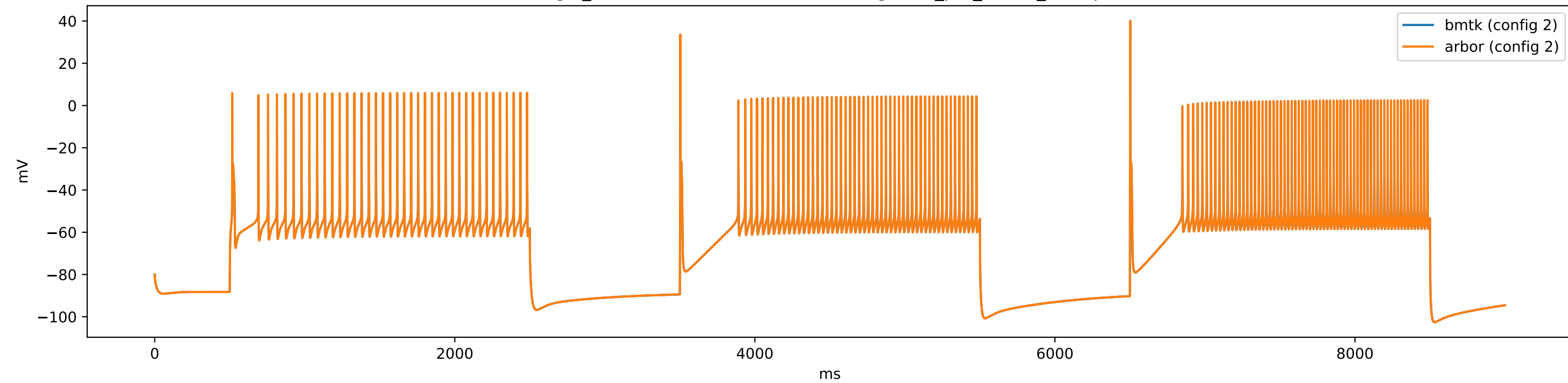
gid_24-475459689 (e4Nr5a1) - config.1cell_per_model_iclamp
