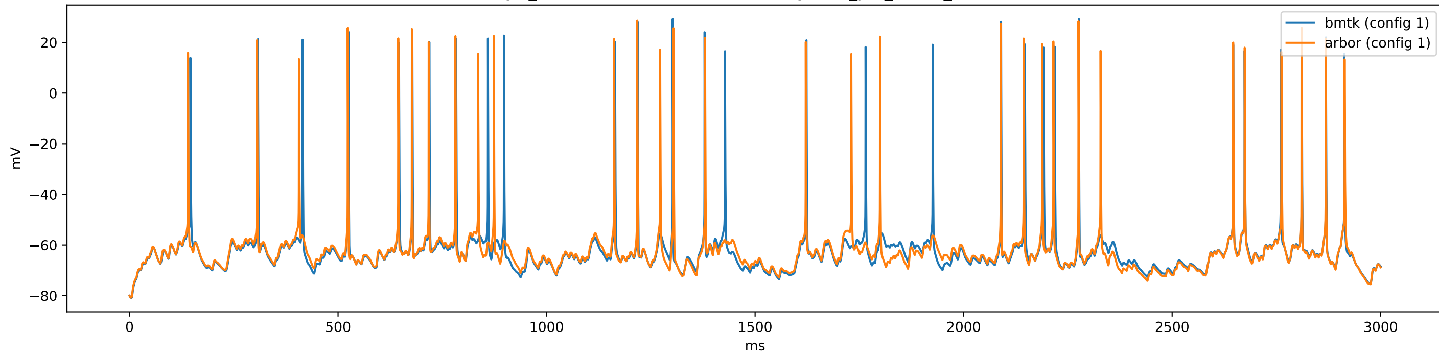
gid_48-487601493 (e4other) - config.1cell_per_model_iclamp
