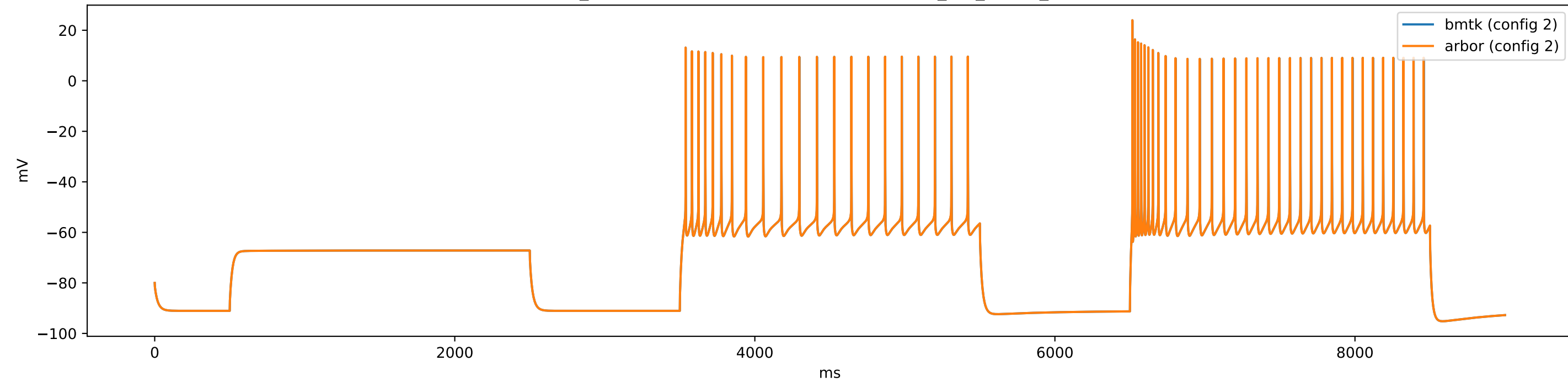
gid_103-471819401 (e6Ntsr1) - config.1cell_per_model_iclamp
