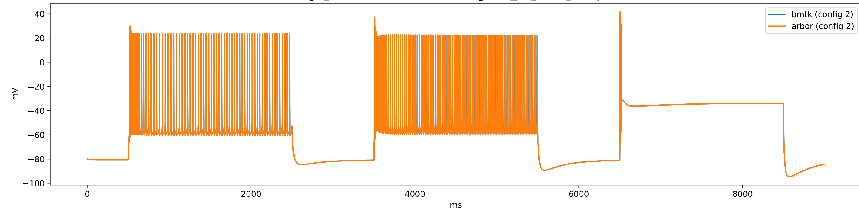
gid_29-329550137 (e4Rorb) - config.1cell_per_model_iclamp
