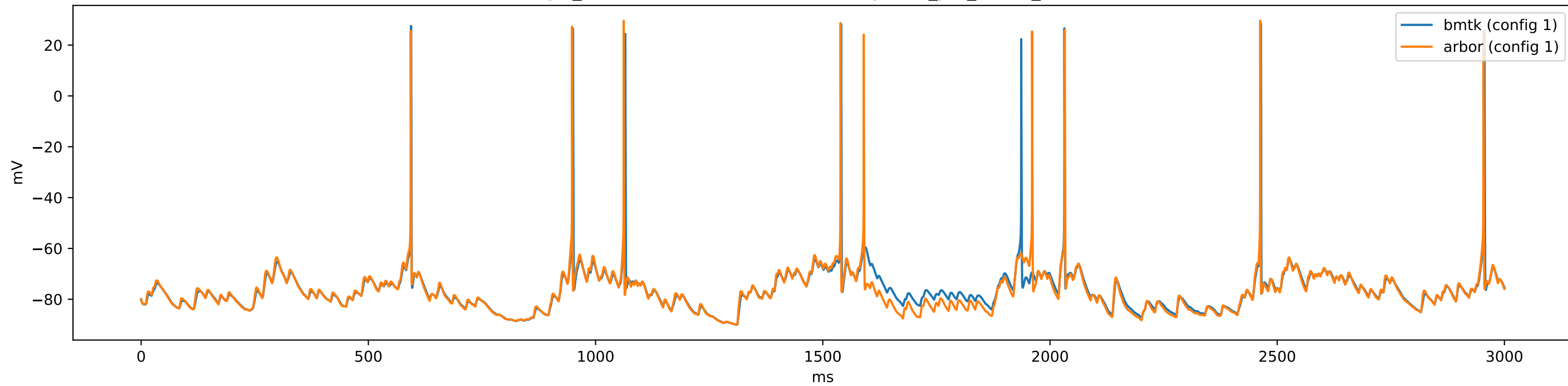
gid_21-386049446 (e4Nr5a1) - config.1cell_per_model_iclamp
