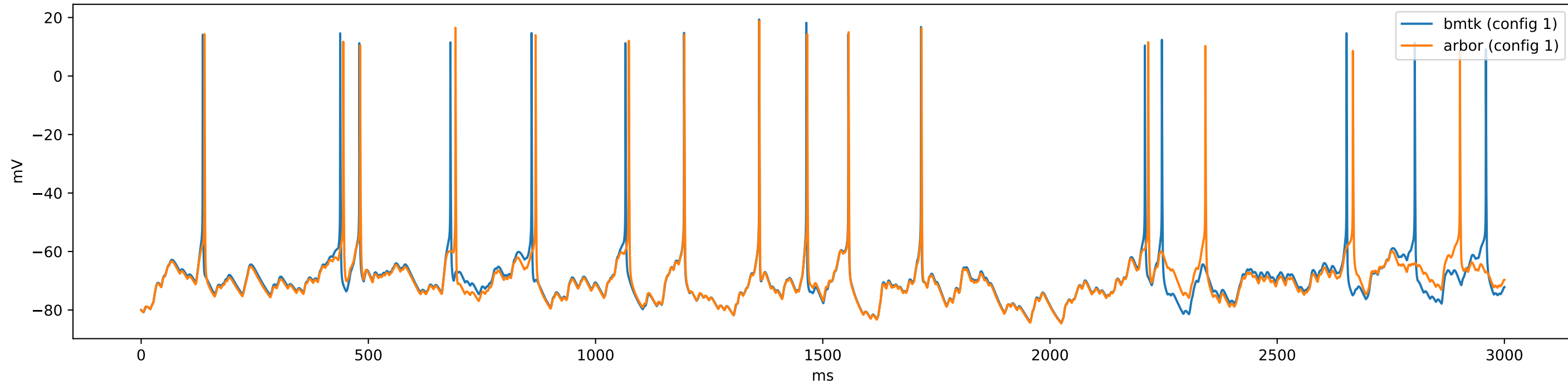
gid_41-469798159 (e4Scnn1a) - config.1cell_per_model_iclamp
