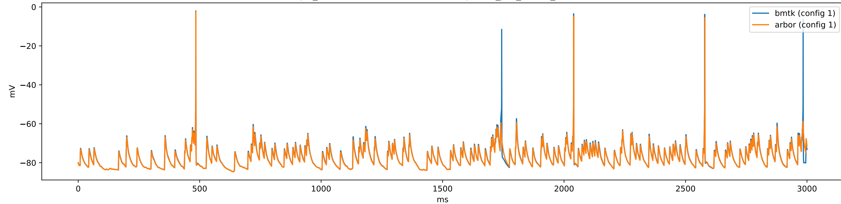
gid_51-487667205 (i4Pvalb) - config.1cell_per_model_iclamp
