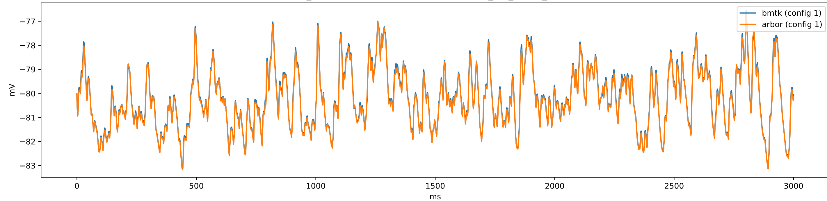
gid_57-471767045 (e5Rbp4) - config.1cell_per_model_iclamp
