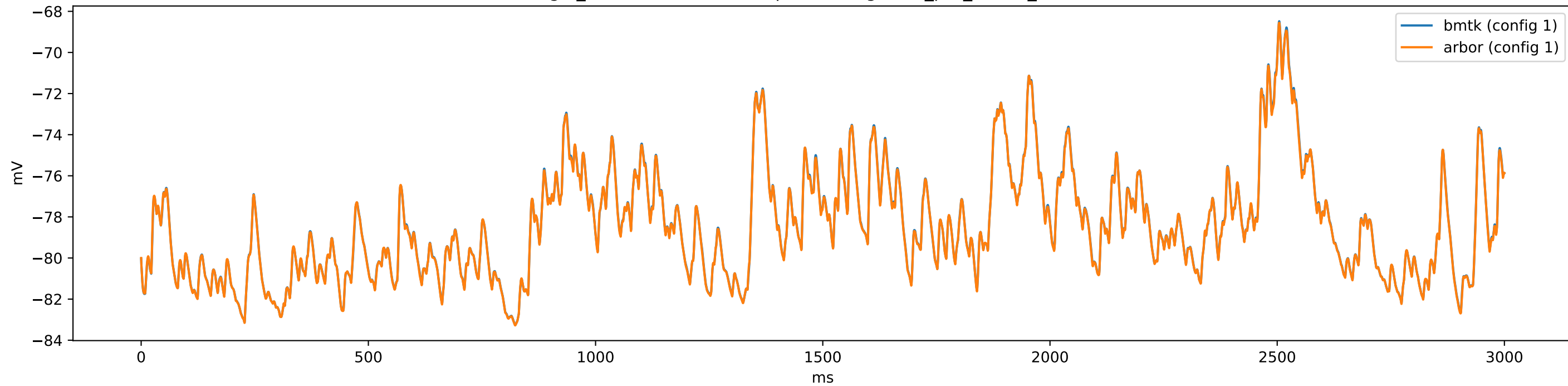
gid_59-485835055 (e5Rbp4) - config.1cell_per_model_iclamp
