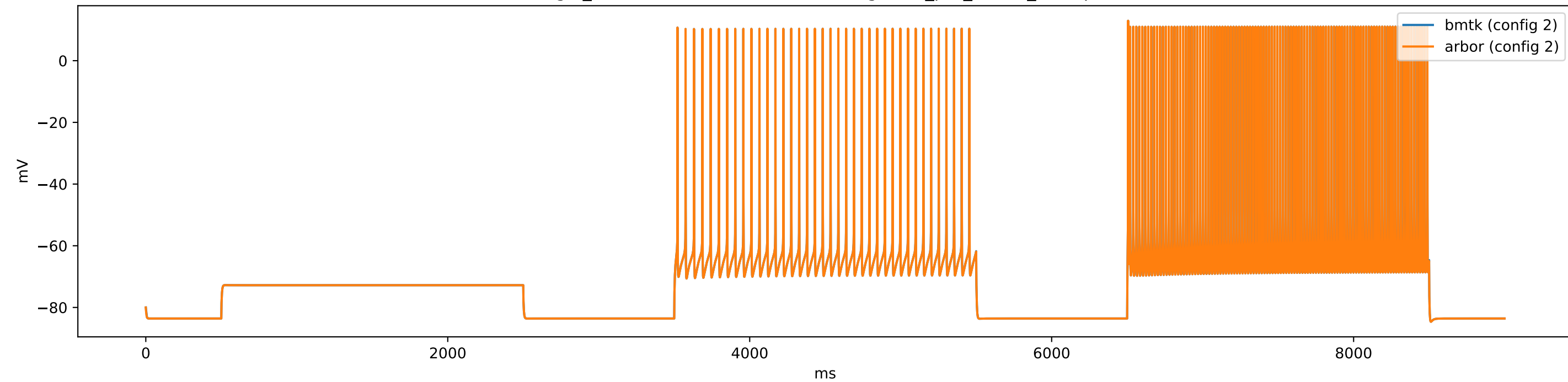
gid_6-473943881 (i23Htr3a) - config.1cell_per_model_iclamp
