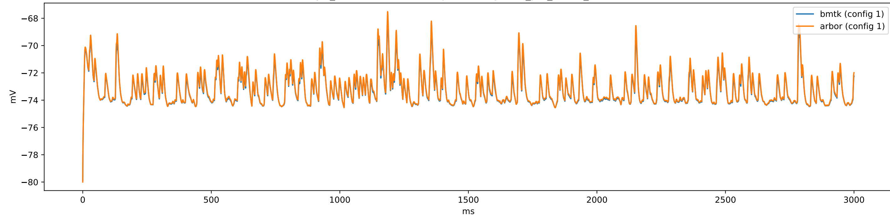
gid_62-486110216 (e5Rbp4) - config.1cell_per_model_iclamp
