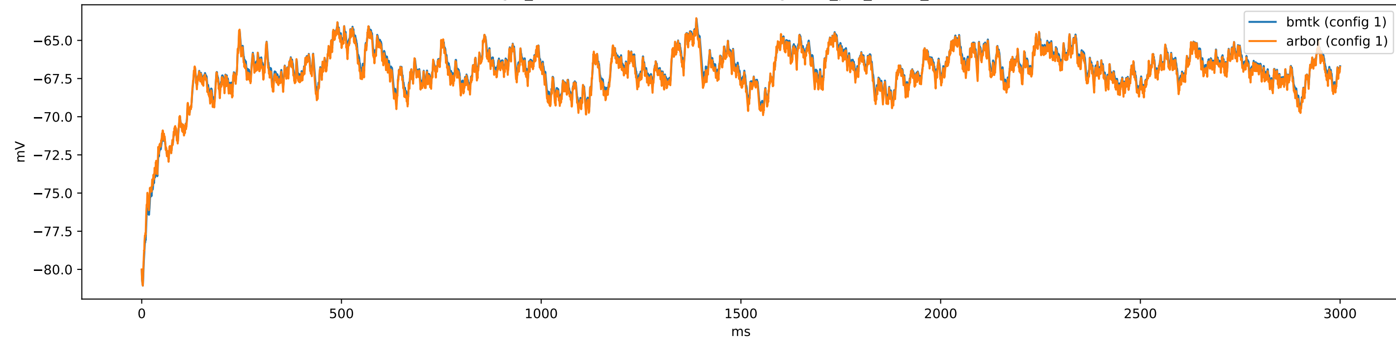
gid_81-478110866 (i5Htr3a) - config.1cell_per_model_iclamp
