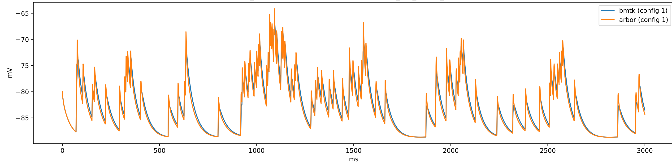
gid_93-486783119 (i5Pvalb) - config.1cell_per_model_iclamp
