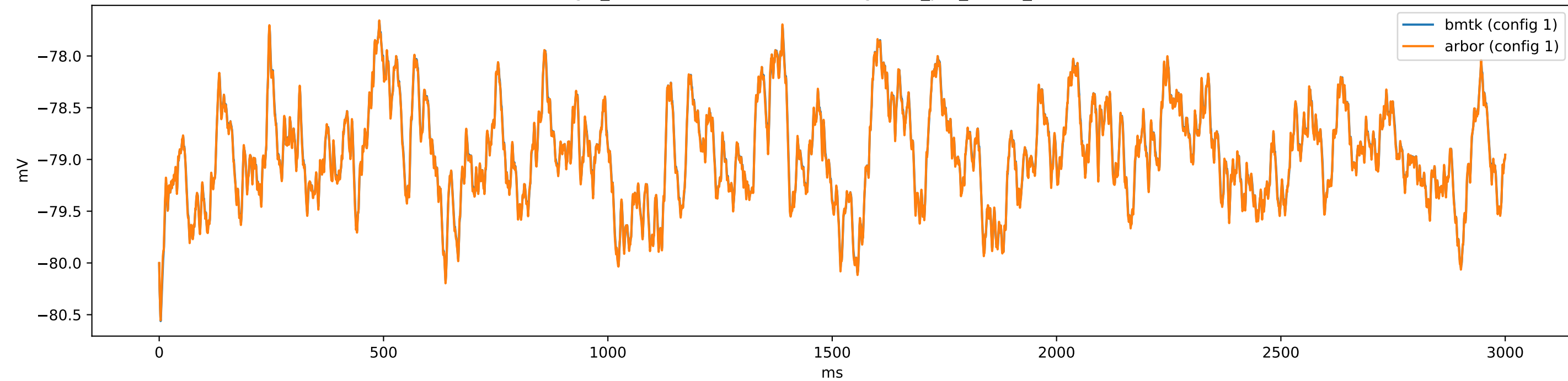
gid_98-482690728 (i5Sst) - config.1cell_per_model_iclamp
