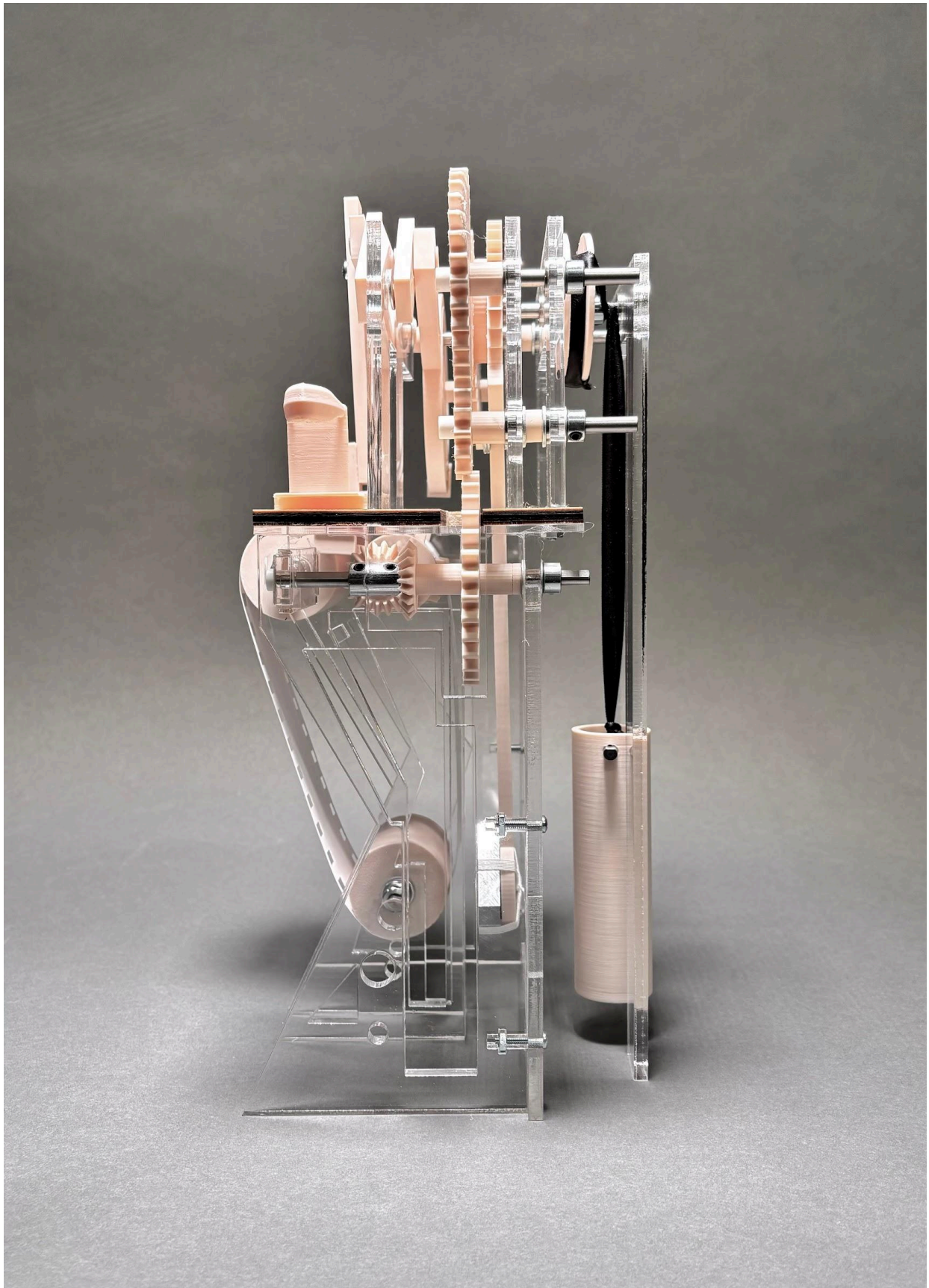
Figure 4: Side (right) view of stamping clock.
