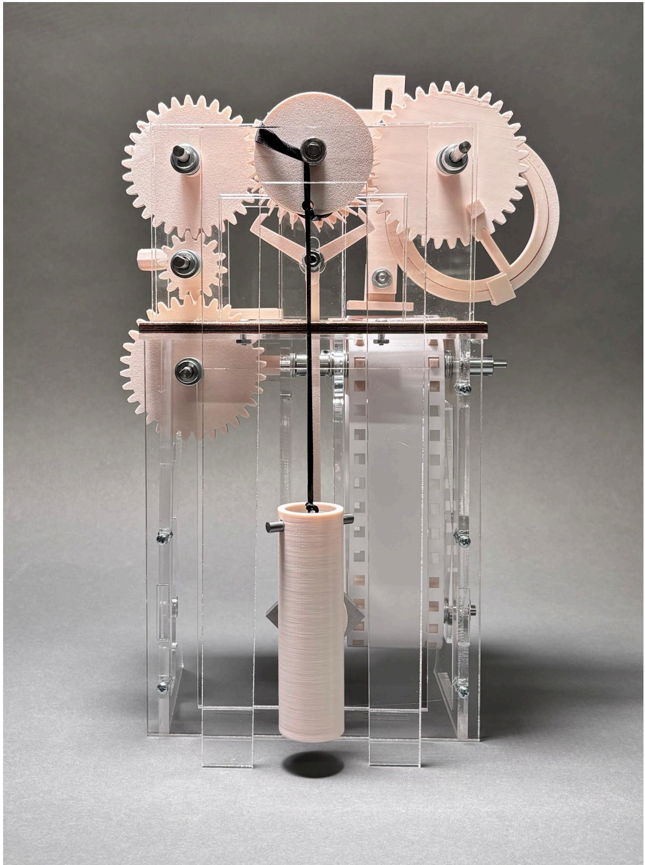
Figure 3: Back view of stamping clock.
