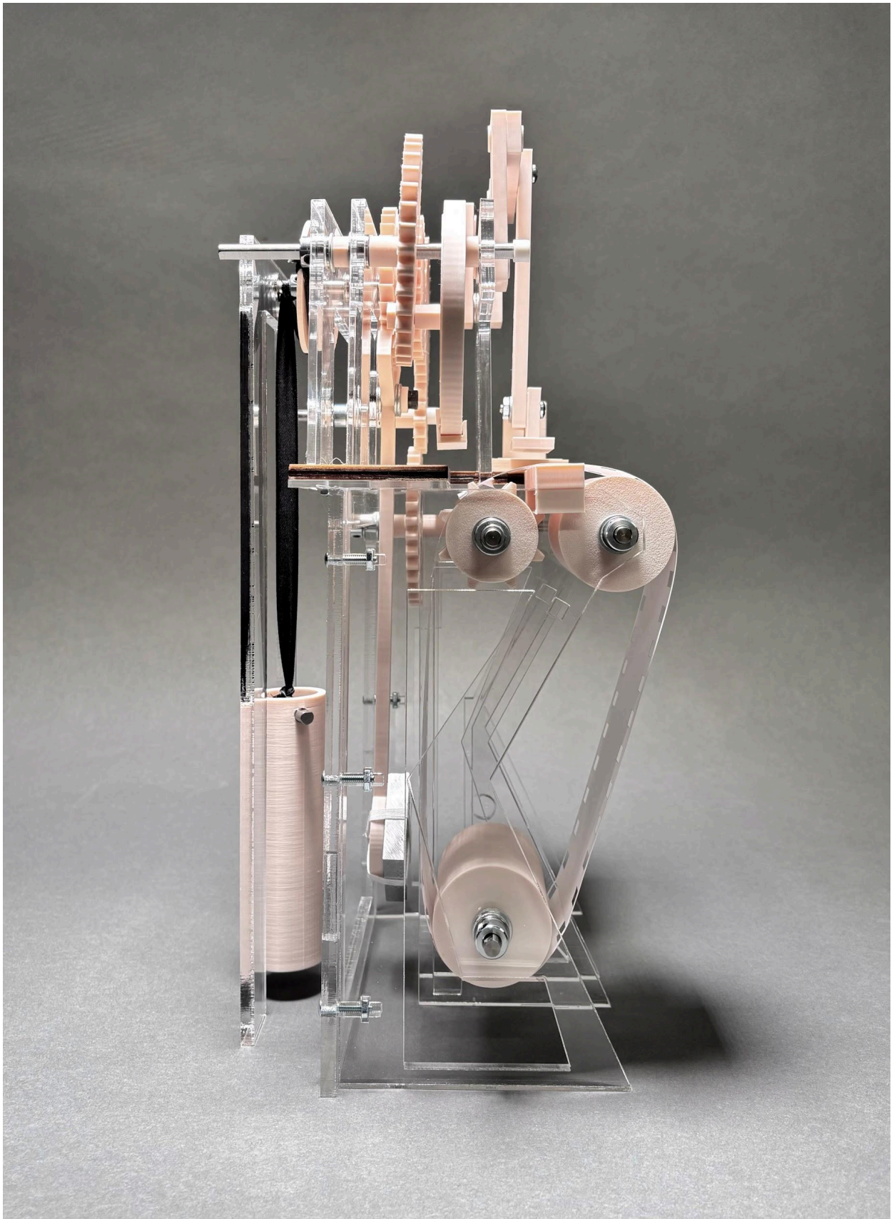
Figure 2: Side (left) view of stamping clock.
