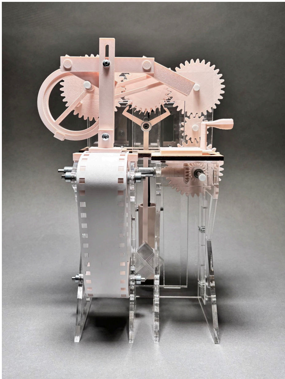
Figure 1: Front view of stamping clock.
