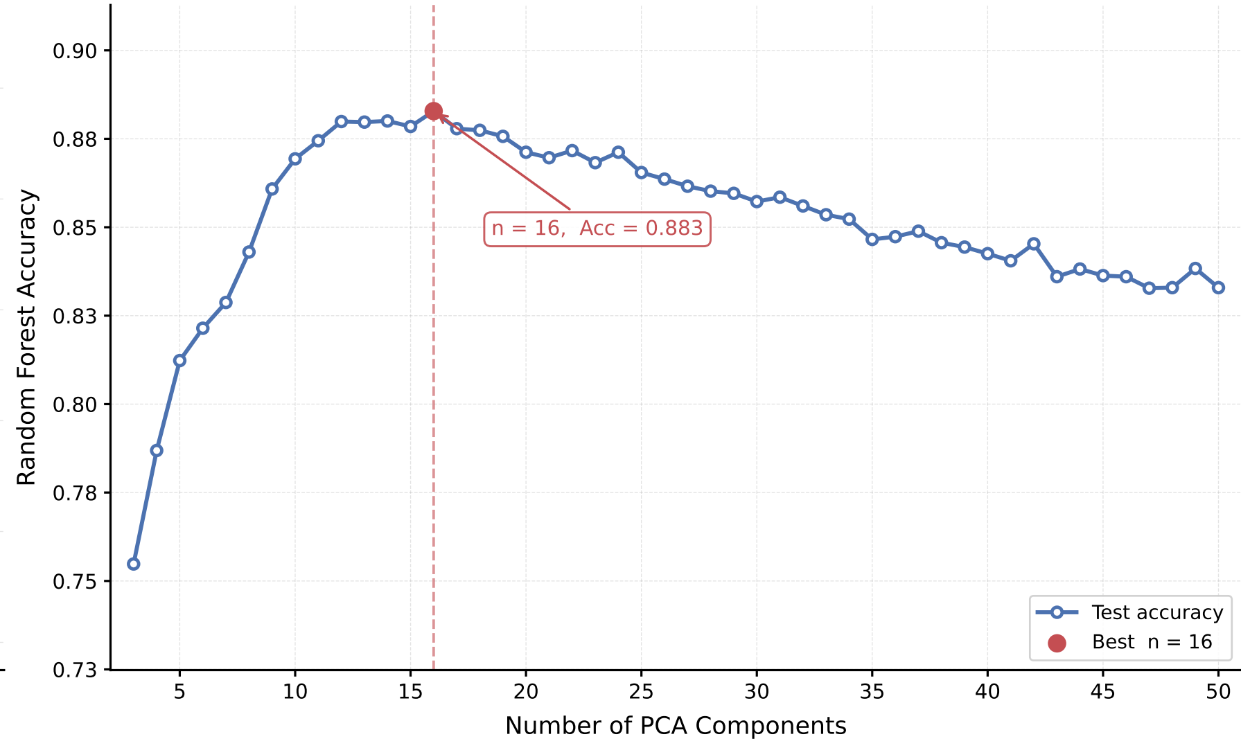
(b) RF Accuracy vs. Number of PCA Components
