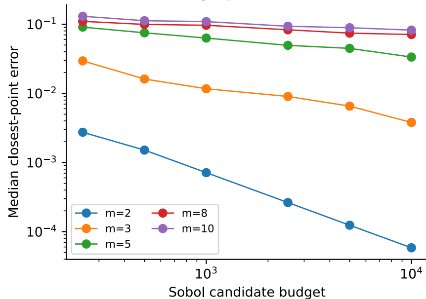
Coverage pilot, 30 seeds
