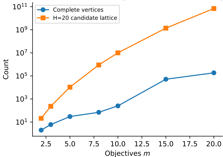
Exact enumeration grows combinatorially
