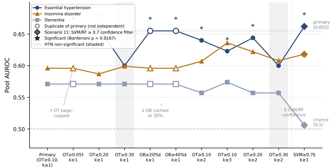
Figure 3. Sensitivity analysis — pool AUROC across 11 scenarios (7 independent + Scenario 11)
