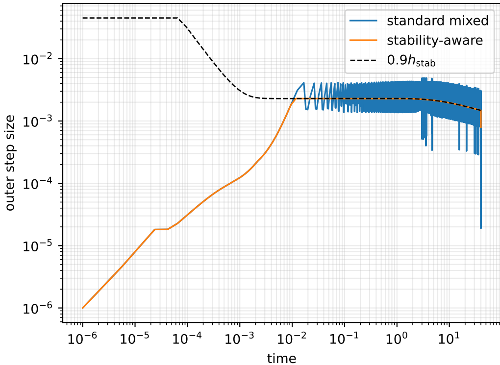
Step histories at tolerance 10^{-6}
