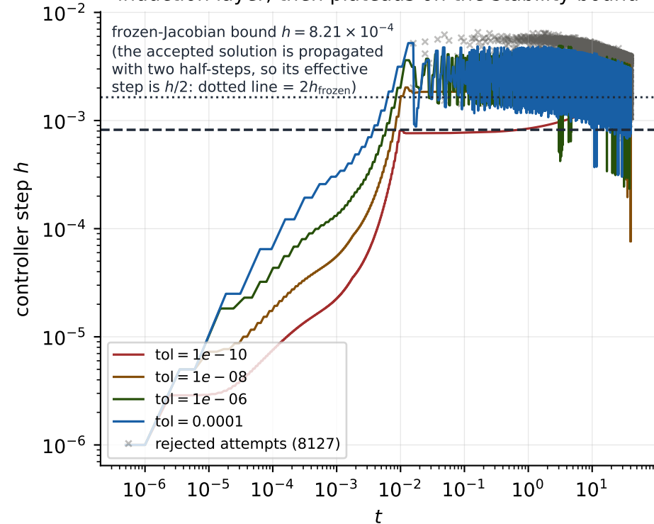
(a) The step size is not constant: it collapses through the induction layer, then plateaus on the stability bound
