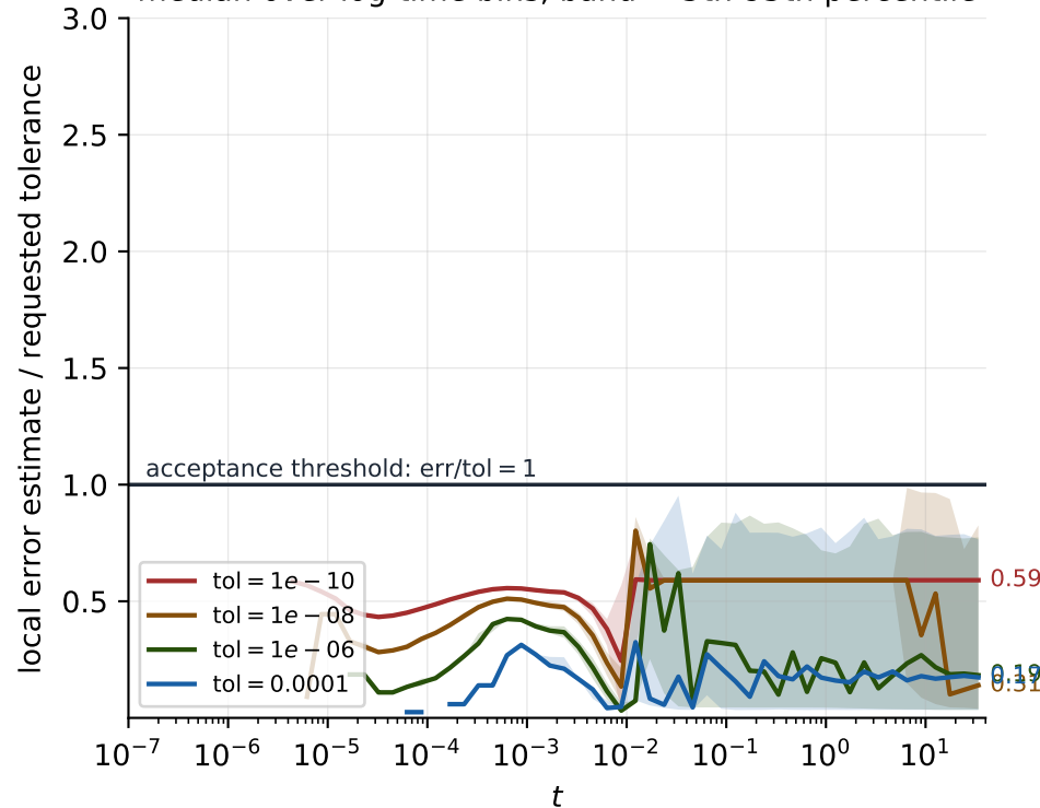
(b) The controlled quantity does track the tolerance median over log-time bins, band = 5th-95th percentile
