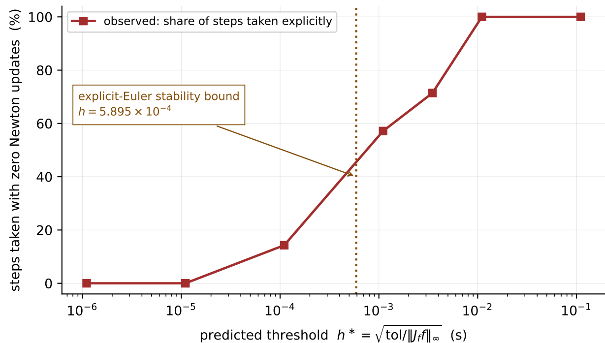
(b) Below the threshold the step is explicit Euler, and above the dotted line that method is unstable
