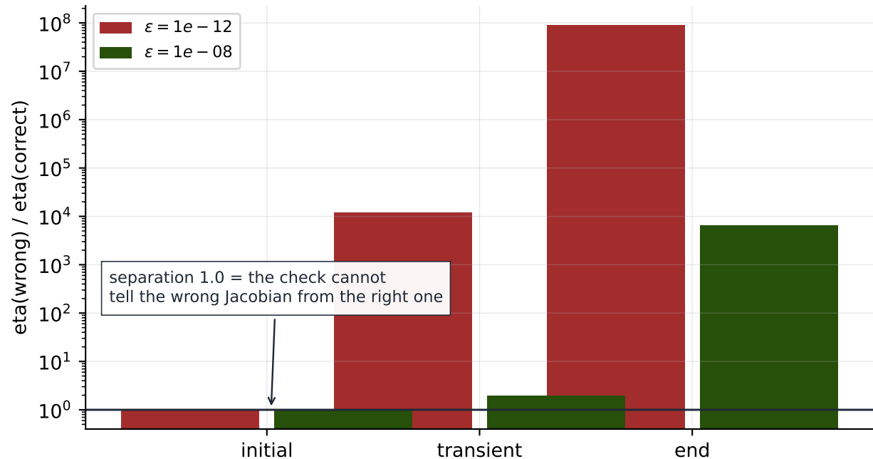
(b) Deleting the whole 10^4 y_2 y_3 reaction at y(0) the check is blind; elsewhere the perturbation decides
