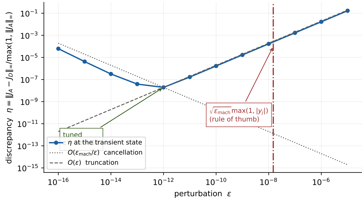
(a) Roundoff on the left, truncation on the right the U-shape is the evidence that the check measures both
