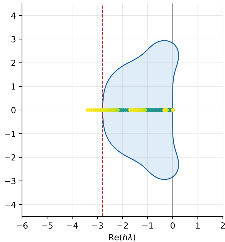
RK4 (order 4) stable real interval [-2.7853, 0]
