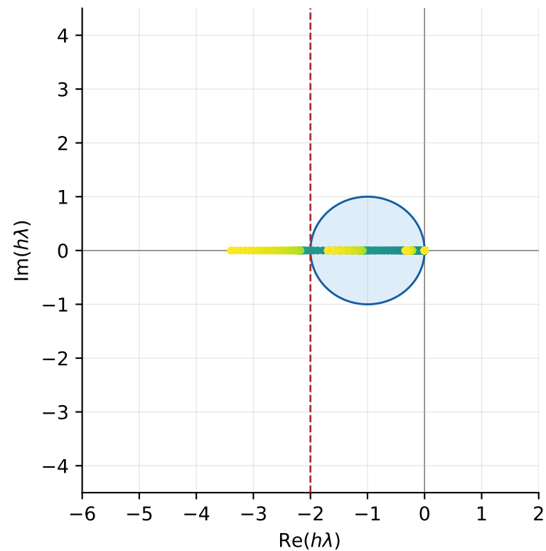
Explicit Euler (order 1) stable real interval [-2.0000, 0]
