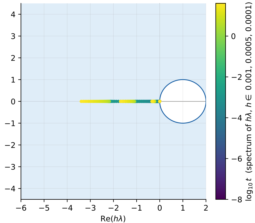
Implicit Euler (order 1) stable real interval unbounded ( \lambda in left half plane) A-stable, L-stable
