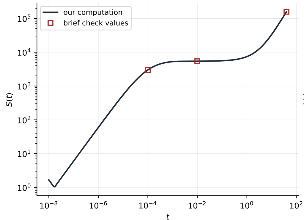
(a) S(t) from the two non-zero eigenvalues only
