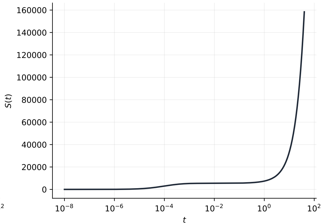
(b) Same data, log-time / linear ratio (growth is concentrated at late t )
