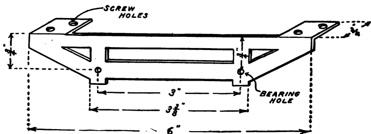
FIG. 265. — Details of the Bearing which supports the Wheel and Axle.
