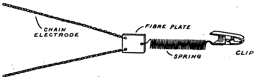
FIG. 127. — Details of the Chain Electrodes, etc.
