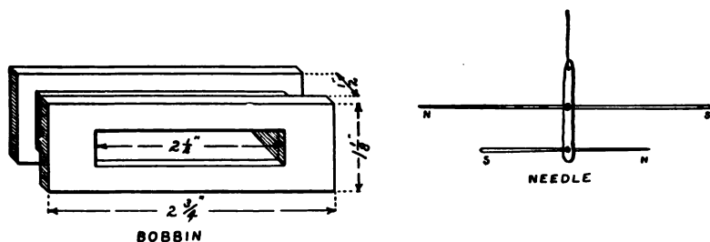
FIG. 114. — Bobbin for Astatic Galvanometer.
