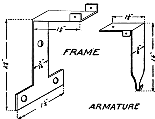
FIG 129. — Details of the Drop-Frame and Armature.
