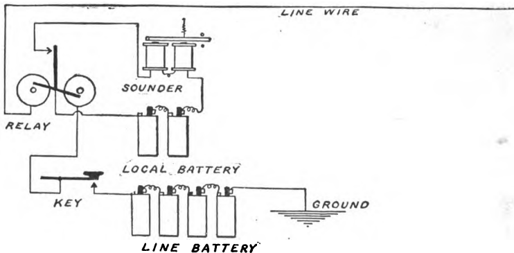
FIG. 140. — A Diagram showing how to connect a Relay, Sounder, and Key.
