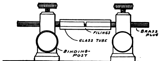
FIG. 234. — Details of the Coherer.
