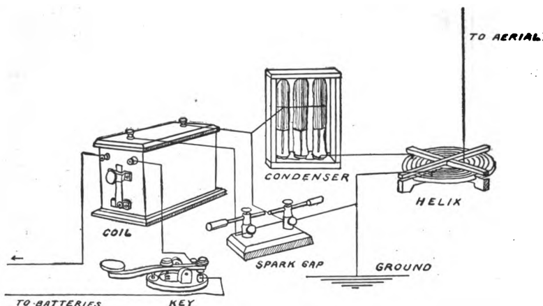
FIG. 228. — Circuit showing how to connect a Helix and a Condenser.
