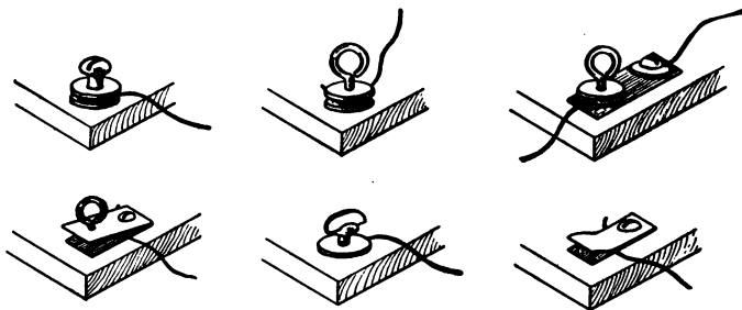
FIG. 93. — Home-made Binding-Posts.
