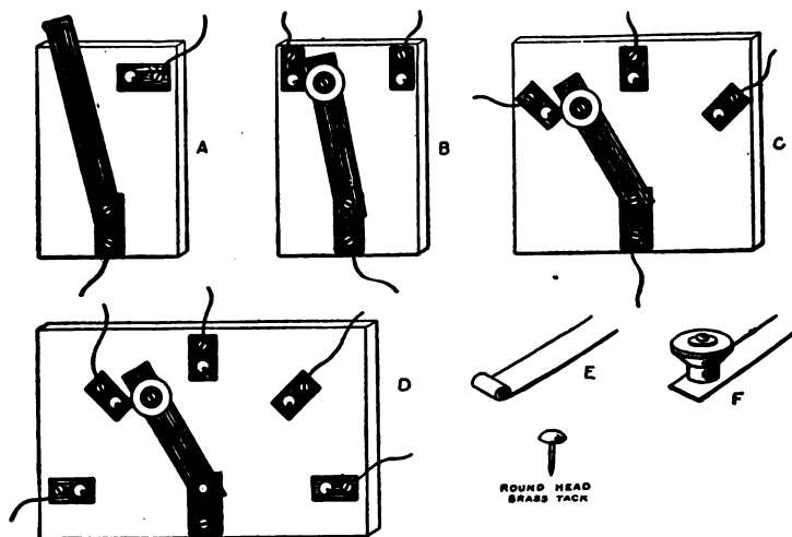
FIG. 95. — Simple Switches.
