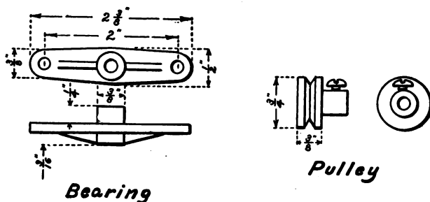
FIG. 260. — The Pulley and Bearings.
