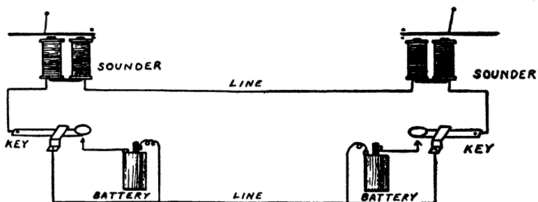
FIG. 134. — A Diagram showing how to connect two Simple Telegraph Stations.
