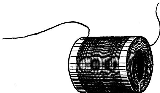
FIG. 163. — Completed Secondary Winding.
