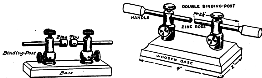
FIG. 222. — Small Spark-Gaps.
