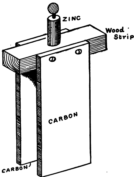
FIG. 61. — An Element made from two Carbon Plates and a Zinc Rod.
