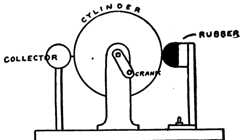
FIG. 29. — Front View of a Cylinder Electric Machine.
