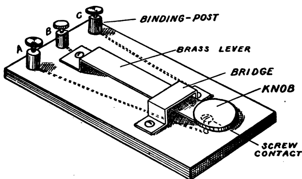
FIG. 132. — A Simple Home-made Telegraph Key.
