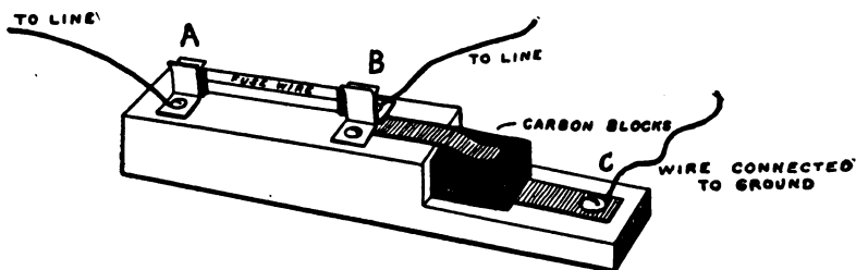
FIG. 101. — Lightning-Arrester for Telephone Wires.
