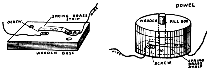
FIG. 123. — Two Simple Push-Buttons.
