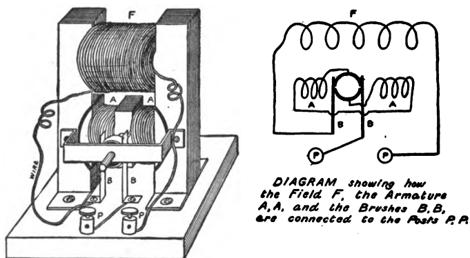
FIG. 250. — Complete Motor.
