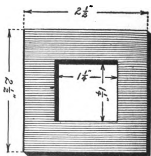
FIG. 183. — Fiber Head.
