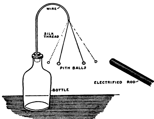
FIG. 23. — A Double Pith-Ball Electroscope.
