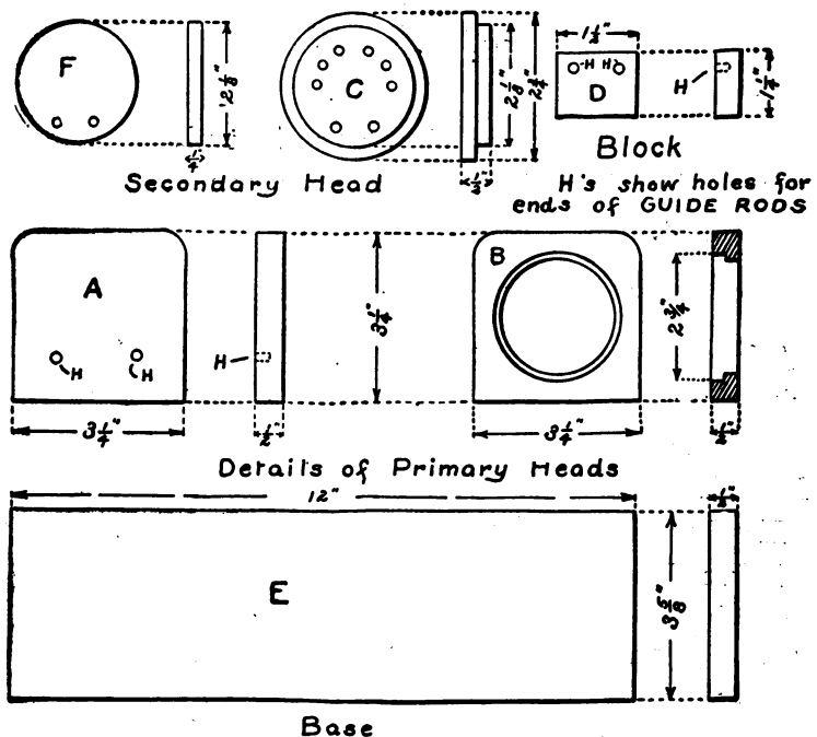
FIG. 205.—Details of the Wooden Parts.
