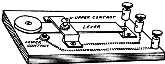
FIG. 239. — A Double-Contact Strap-Key.
