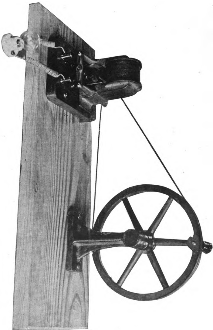
THE JUNIOR DYNAMO MOUNTED ON A LONG WOODEN BASE AND BELTED TO A GROOVED WHEEL, FITTED WITH A CRANK SO THAT THE DYNAMO CAN BE RUN AT HIGH SPEED BY HAND POWER. THE ILLUSTRATION ALSO SHOWS A SMALL INCANDESCENT LAMP CONNECTED TO THE DYNAMO SO THAT WHEN THE CRANK IS TURNED THE LAMP WILL LIGHT.
