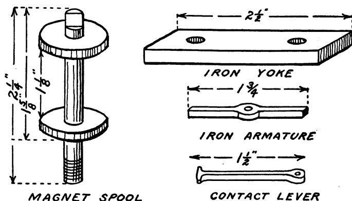
FIG. 138. — Details of the Relay Parts.
