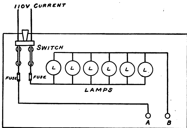
FIG. 312. — Top View of Lamp Bank, showing how the Circuit is arranged.
