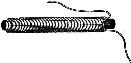
FIG. 160. — Complete Primary Winding and Core.
