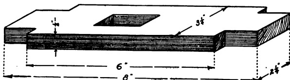
FIG. 264. — Details of the Floor of the Car.
