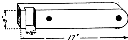
FIG. 38. — The Upright.
