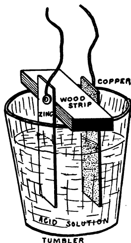
FIG. 54. — A Home-Made Voltaic Cell.
