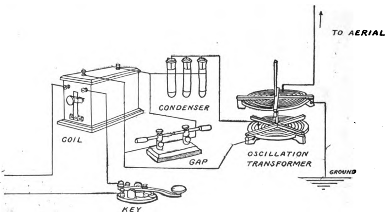
FIG. 229. — Circuit showing how to connect an Oscillation Transformer and a Condenser.
