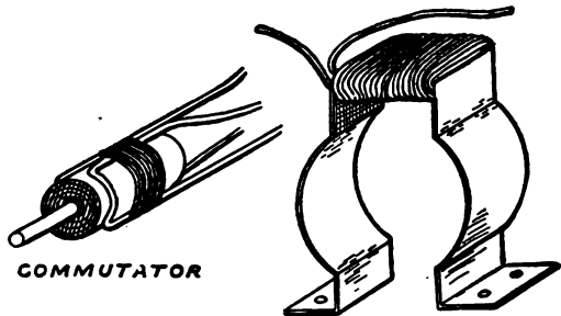
FIG. 246. — The Field and Commutator.
