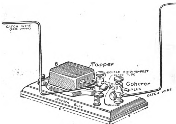
FIG. 233. — A Coherer and a Decoherer.
