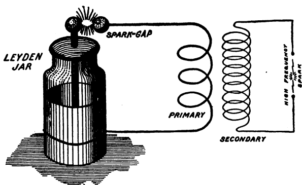
FIG. 317. — Illustrating the Principle of the Tesla Coil.
