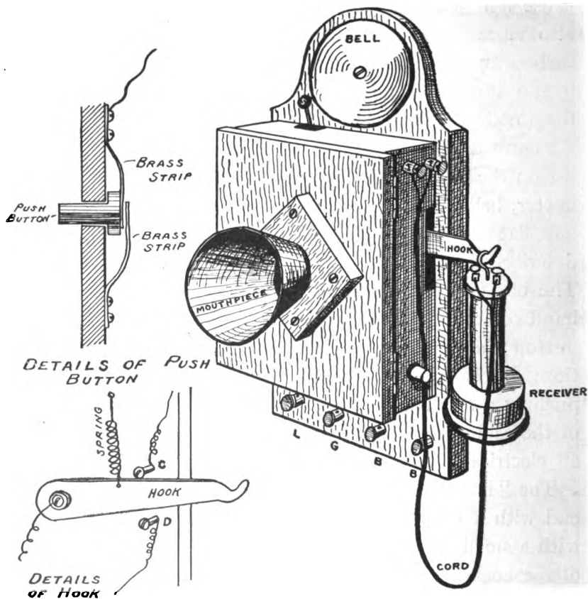
FIG. 149. — A Complete Telephone Instrument.
