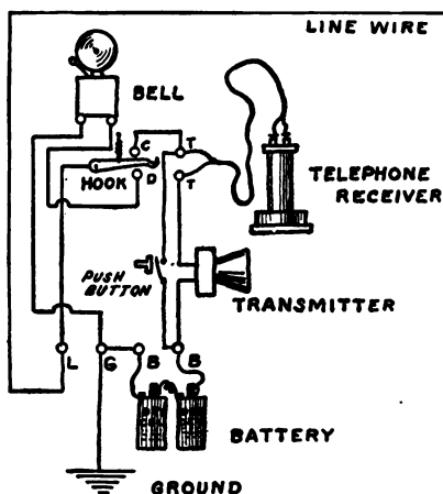
FIG. 150. — Diagram of Connection for the Telephone Instrument shown in Fig. 149.
