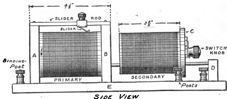
FIG. 206. — Side View of the Loose Coupler.
