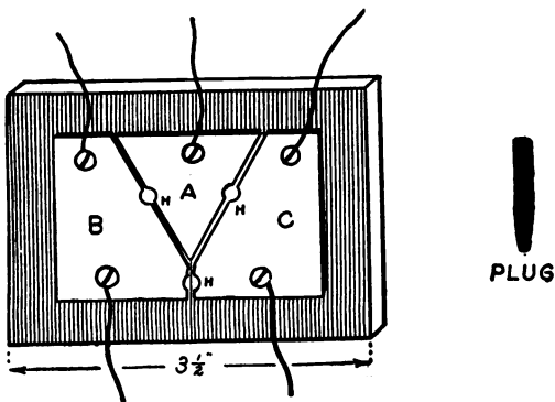
FIG. 100. — Home-made Lightning-Arrester.
