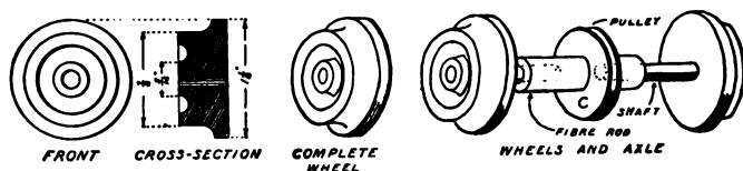
FIG. 266. — The Wheels and Axle.
