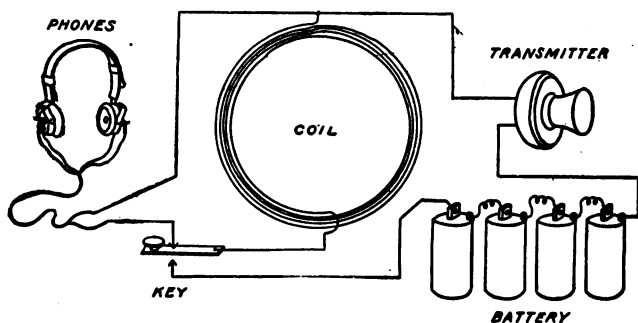
FIG. 240. — The Circuit of the Wireless Telephone.
