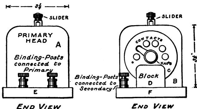
FIG. 208. — End Views of the Loose Coupler.
