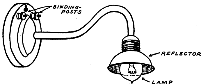
FIG. 290. — A Lamp Bracket for Miniature Lighting.
