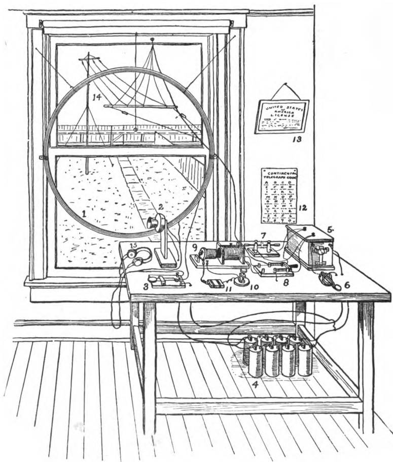
FIG. 241. — A Complete Wireless Telephone and Telegraph Station for Amateurs.
