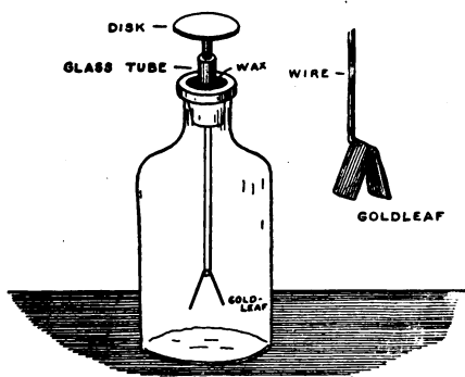
FIG. 24. — A Gold-Leaf Electroscope.
