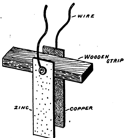
FIG. 53. — The Elements of Simple Voltaic Cell.
