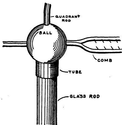
FIG. 41. — Showing how the Ball, Comb, etc., are mounted on the Glass Rod.
