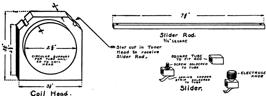
FIG. 201. — Details of the Tuning Coil.
