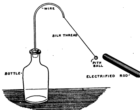
FIG. 22. — A Pith-Ball Electroscope.
