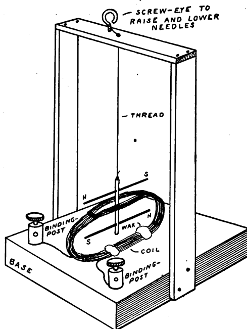
FIG. 112. — Astatic Galvanoscope.
