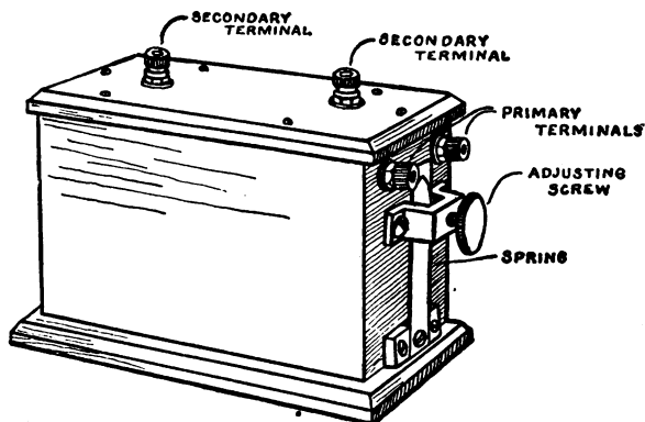
FIG. 221. — A Wireless Spark Coil.
