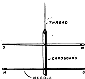
FIG. 113. — Astatic Needles.
