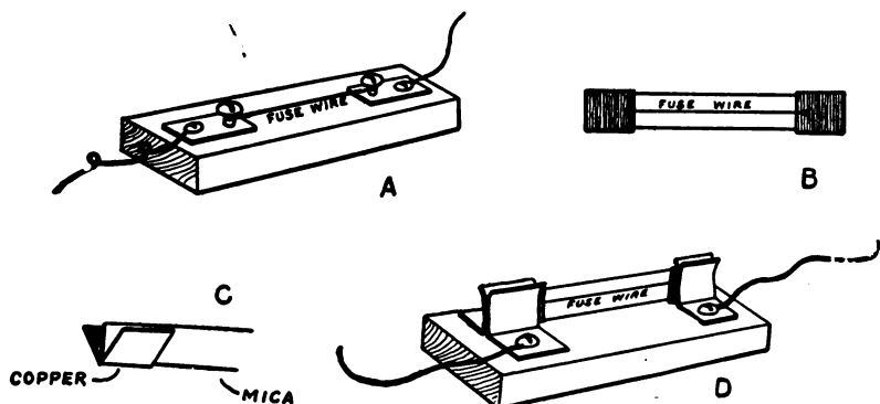
FIG. 98. — Simple Fuses.
