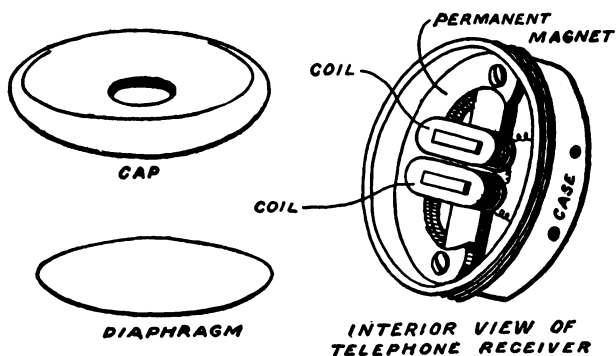
FIG. 146. — A Watch-Case Telephone Receiver.
