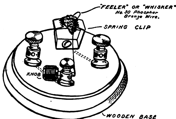
FIG. 212. — Details of the "Cat-Whisker" Detector.
