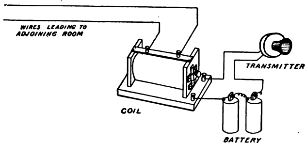
FIG. 167. — Diagram showing how to connect the Apparatus for the "Elect Hands" Experiment.
