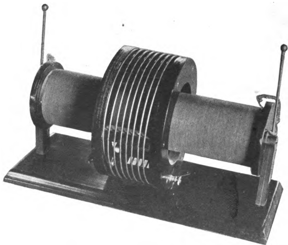
THE TESLA HIGH-FREQUENCY COIL.
