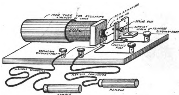
FIG. 156. — Completed Medical Coil.
