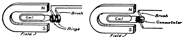
FIG. 252. — The Principle of the Alternator and the Direct-Current Dynamo.
