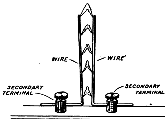
FIG. 171. — Jacob's Ladder.
