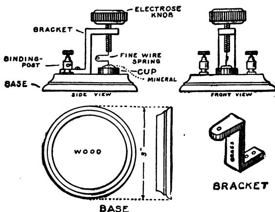
FIG. 211. — Details of the Crystal Detector.
