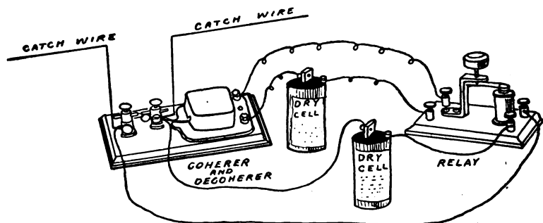
FIG. 236. — The Complete Coherer Outfit.
