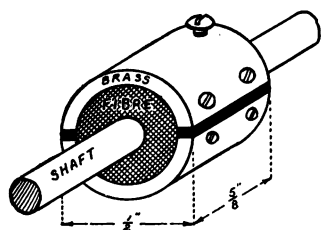
FIG. 257.—Details of the Commutator.
