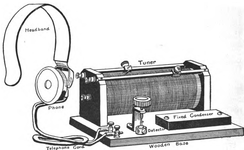
FIG. 316. — A Complete Wireless Receiving Outfit.
