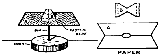
FIG. 21. — A Paper Electroscope.
