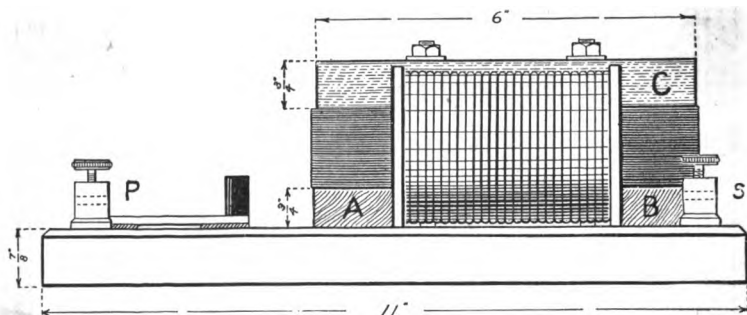
FIG. 192. — Side View of the Transformer.
