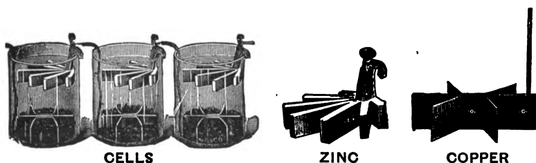
FIG. 75. — Gravity Cells.
