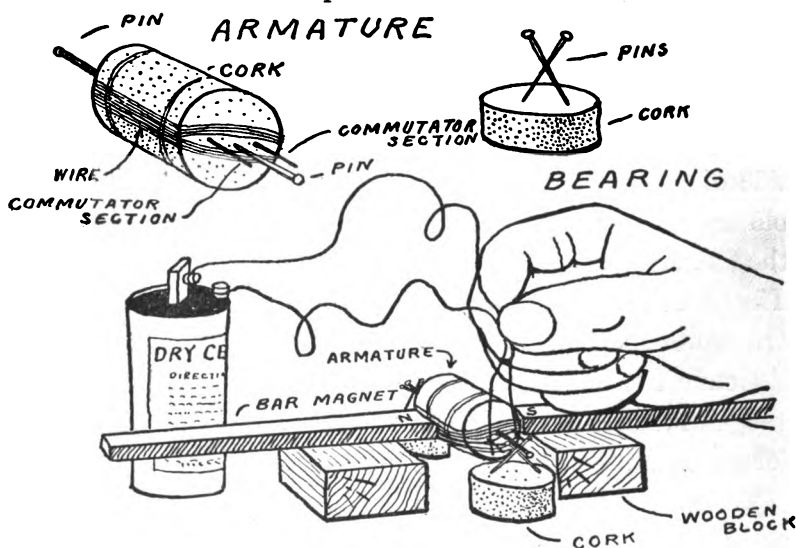
FIG. 242. — A Simple Electric Motor which may be made in Fifteen Minutes.
