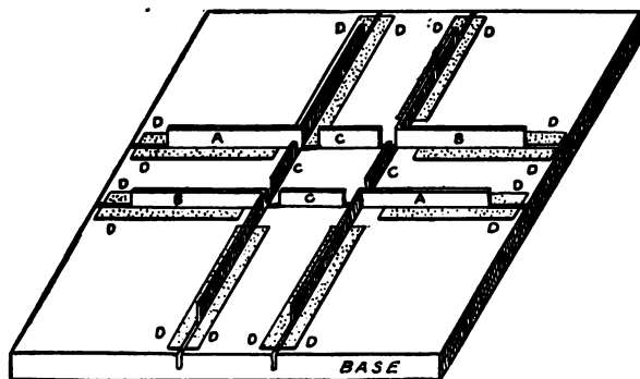
FIG. 276. — The Completed Cross-over.
