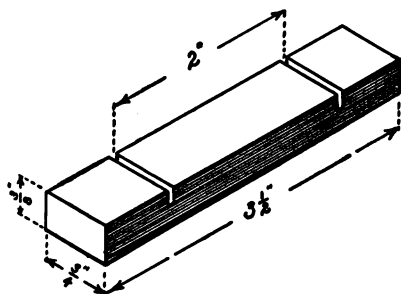
FIG. 272. — Details of a Wooden Tie.
