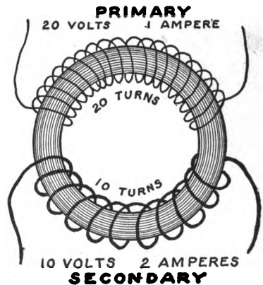
FIG. 179. — Step-Down Transformer.
