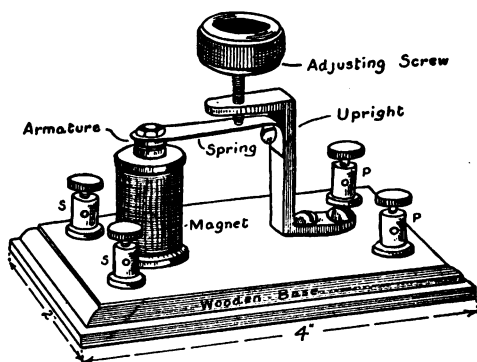
FIG. 235. — The Relay.
