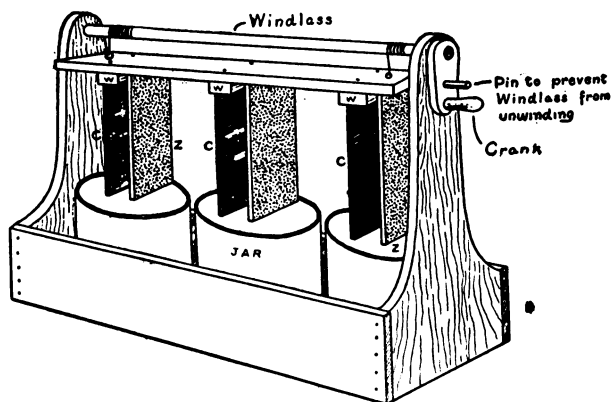
FIG. 64. — A Plunge Battery, with Windlass.
