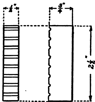
FIG. 319. — Details of the Cross Bars which support the Primary Winding.
