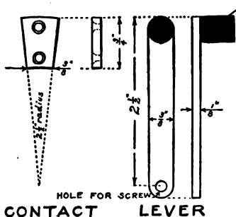
FIG. 188. — Details of the Switch Parts.
