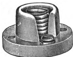
FIG. 284. — Miniature Flat-Base Porcelain Receptacle.
