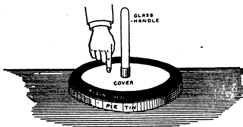
FIG. 27. — The Electrophorus.
