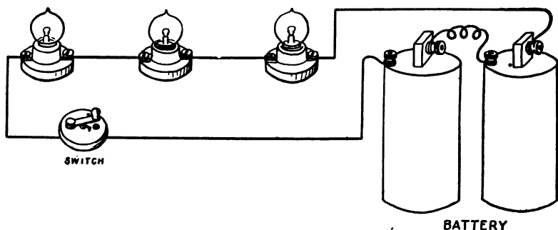
FIG. 288. — How Lamps are Connected in Series.
