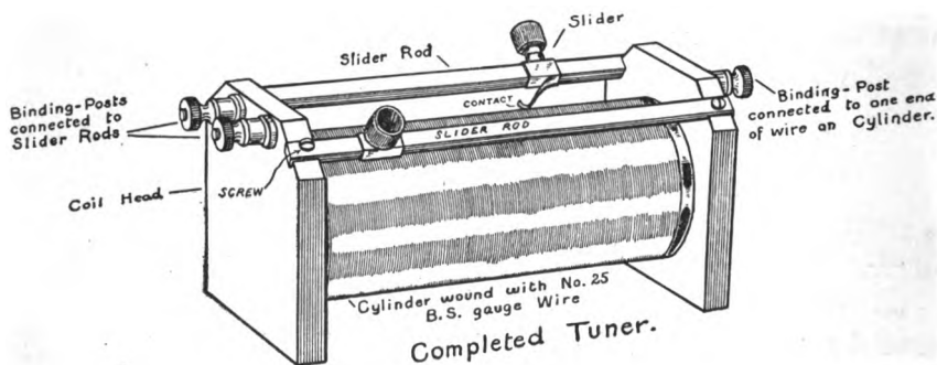
FIG. 203. — Complete Double-Slider Tuning Coil.
