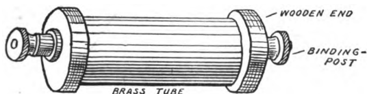
FIG. 216. — A Fixed Condenser enclosed in a Brass Case it together. made from a Piece of Tubing fitted with Wooden Ends.
