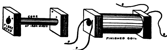
FIG. 152. — A Telephone Induction Coil.
