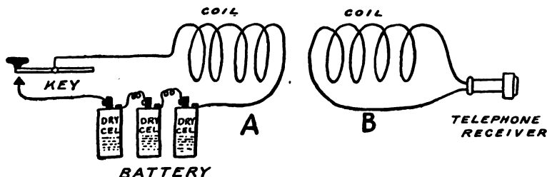
FIG. 237.—A Simple Arrangement showing the Inductive Action between two Coils.
