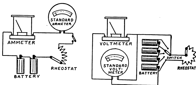
FIG. 109. — Circuits for Calibrating the Ammeter and Voltmeter.
