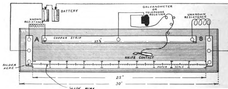
FIG. 116. — Wheatstone Bridge.
