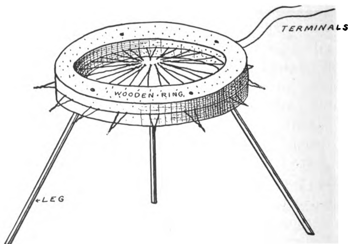
FIG. 305. — Complete Thermopile.
