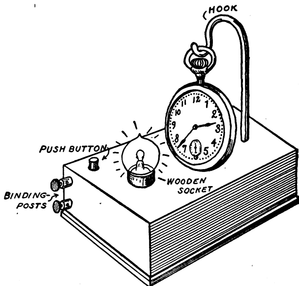
FIG. 299. — A Watch-Light.
