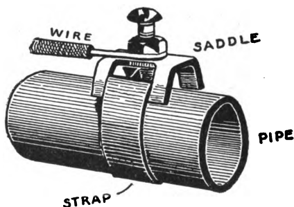
FIG. 200. — A Ground Clamp for Pipes.
