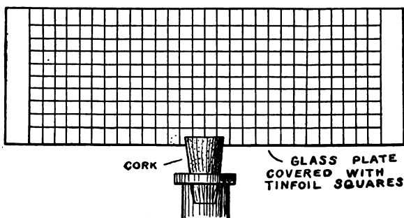
FIG. 48. — A Lightning Board.
