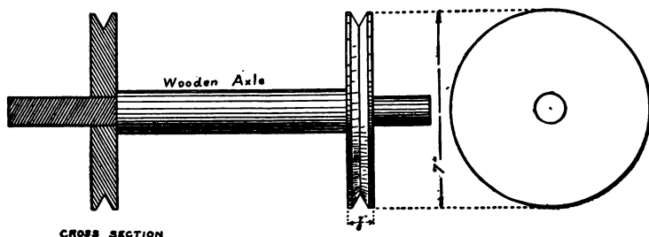
FIG. 39. — The Driving-Wheels and Axle.
