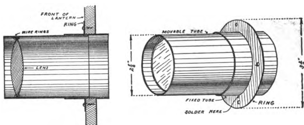
FIG. 307. — How the Lens is Arranged and Mounted.
