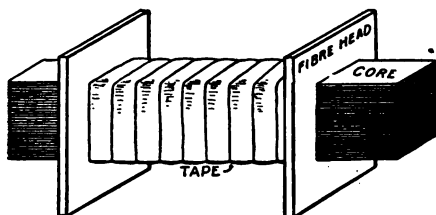
FIG. 184. — Leg with Heads in Position for Winding.
