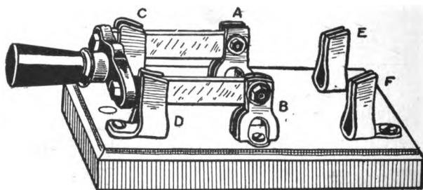
FIG. 230. — An Aerial Switch.
