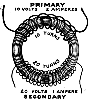
FIG. 178. — Step-Up Transformer.
