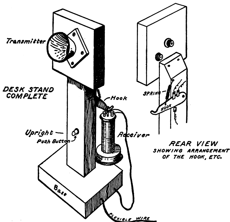
FIG. 151. — A Desk-Stand Type of Telephone.
