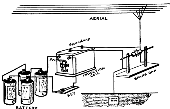
FIG. 194. — A Simple Transmitter.
