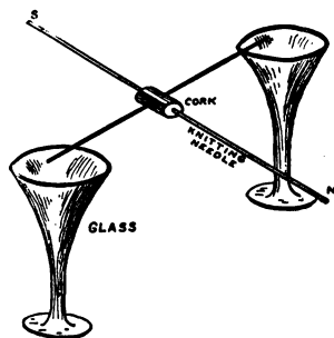
FIG. 16. — A Simple Dipping Needle.
