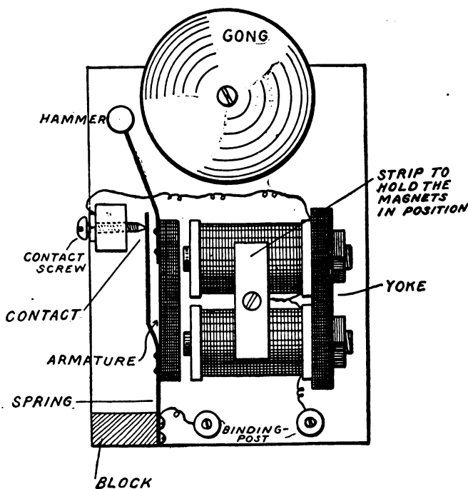
FIG. 121. — The Completed Bell.
