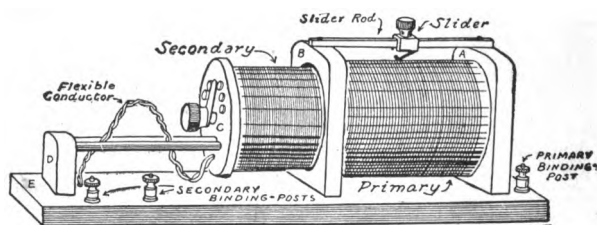
FIG. 209. — Complete Loose Coupler.
