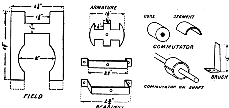
FIG. 249. — Details of the Motor.
