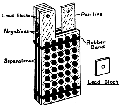
FIG. 73. — The Complete Element for a Storage Cell.
