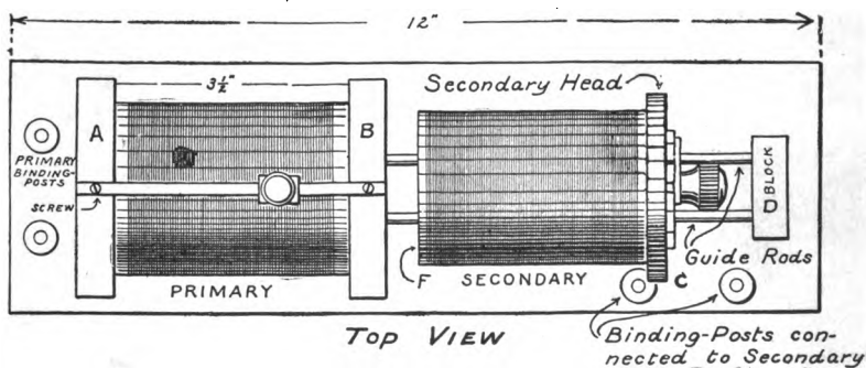
FIG. 207. — Top View of the Loose Coupler.
