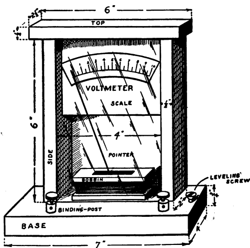
FIG. 108. — Completed Voltmeter.
