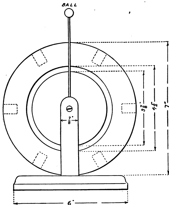
FIG. 321. — End View of the Complete Tesla Coil.
