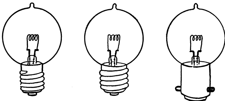
FIG. 283. — Lamps fitted respectively with Miniature, Candelabra, and Ediswan Bases.
