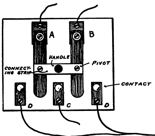
FIG. 315. — A Pole-Changing Switch or Current Reverser.
