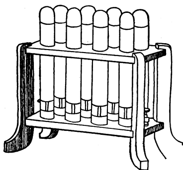
FIG. 225. — Eight Test-Tube Leyden Jars mounted in a Wooden Rack.
