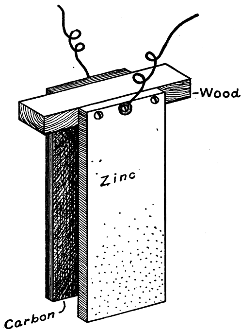
FIG. 59. — A Zinc-Carbon Element, made from Heavy Plates.
