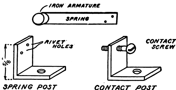
FIG. 155. — Details of Interrupter for Medical Coil.
