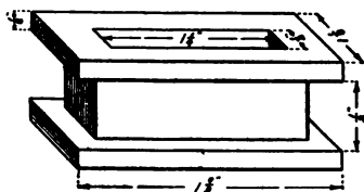
FIG. 106. — Details of the Bobbin.
