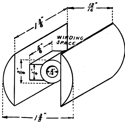
FIG. 256. — Details of the Armature Casting.
