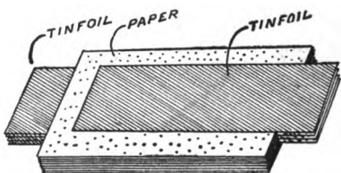
FIG. 215. — Building up a Fixed Condenser.
