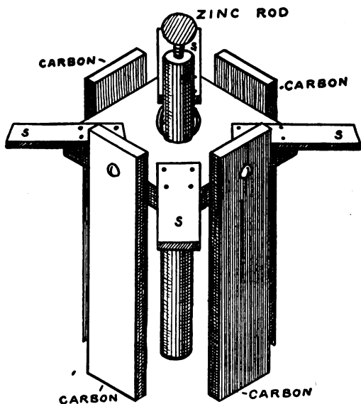
FIG. 62. — A Method of Mounting four Carbon Plates.
