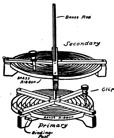
FIG. 227. — An Oscillation Transformer.
