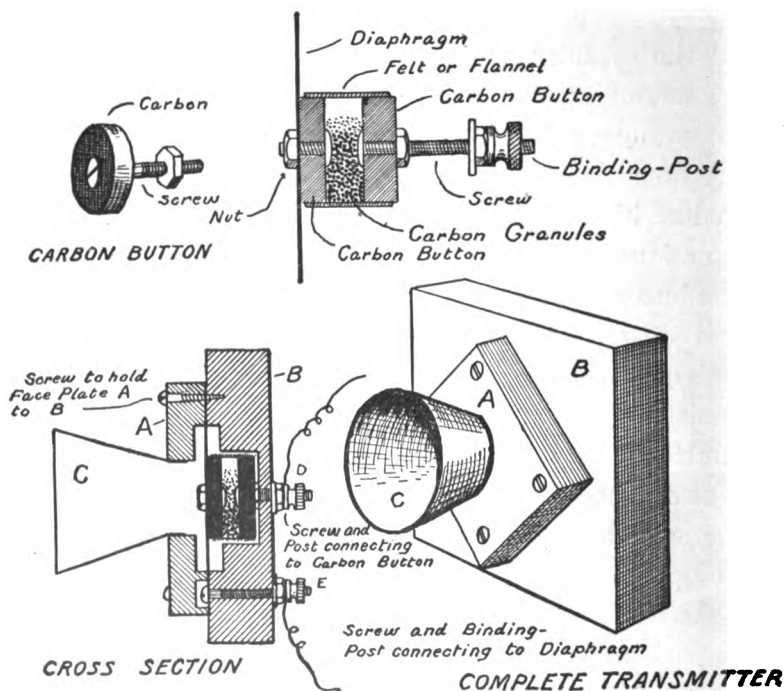
FIG. 148. — A Home-made Telephone Transmitter.
