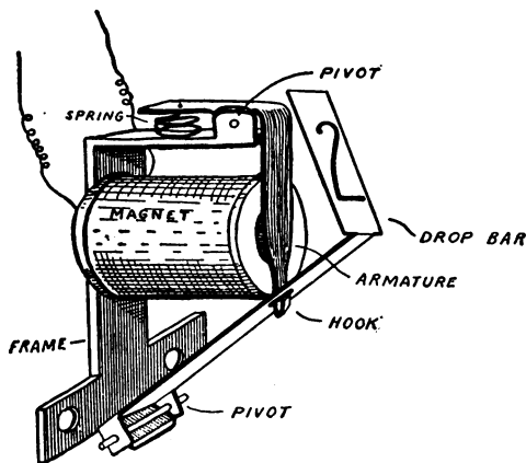
FIG. 128. — An Annunciator Drop.
