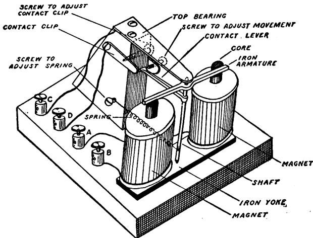
FIG. 139. — The Completed Relay.
