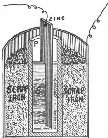
FIG. 67. — A Tomato-Can Cell; Sectional View.
