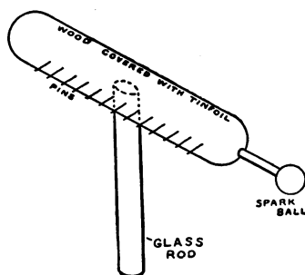
FIG. 32. — The Prime Conductor or Collector.
