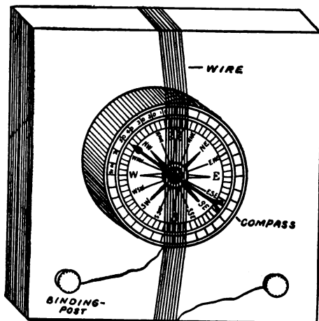
FIG. 110. — Simple Compass Galvanoscope.
