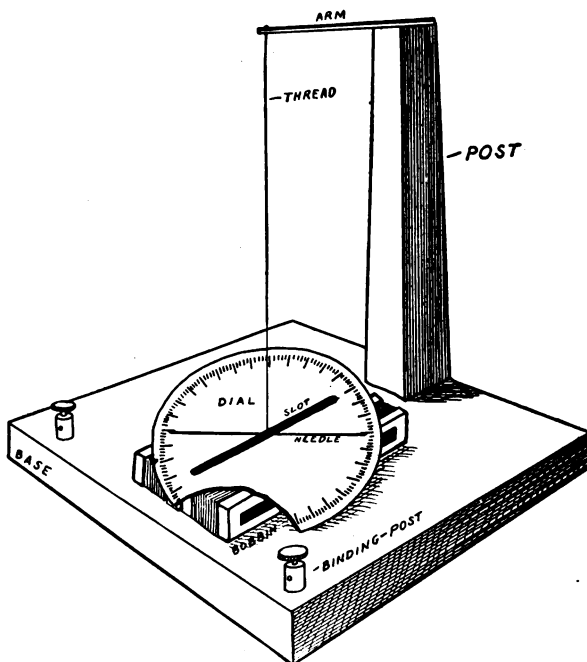
FIG. 115. — Completed Astatic Galvanometer.
