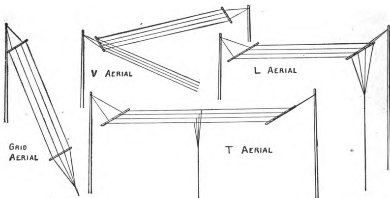
FIG. 199. — Various Types of Aerials.
