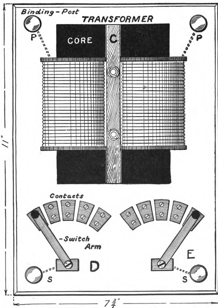
FIG. 191. — Top View of the Transformer.
