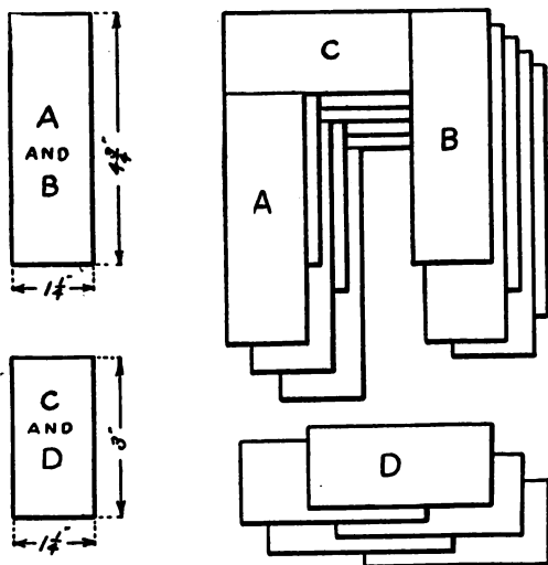
FIG. 180.—Core Dimensions.
