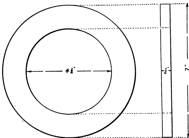
FIG. 318. — Details of the Wooden Rings used as the Primary Heads.
