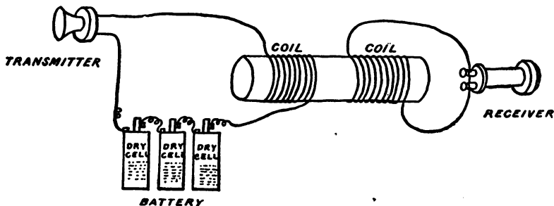
FIG. 238.—A Simple Wireless Telephone.
