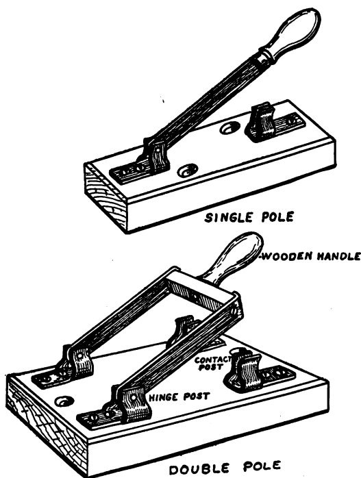
FIG. 96. — Knife Switches.
