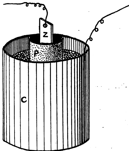
FIG. 68. — The Tomato-Can Cell Complete.
