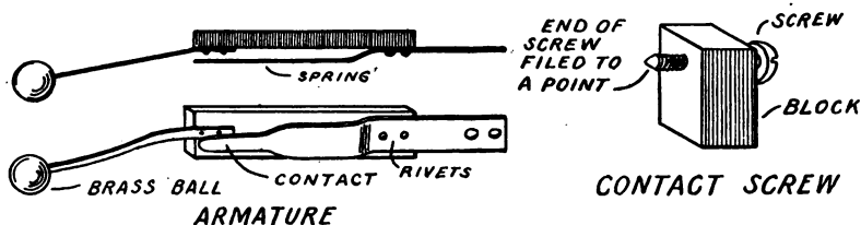
FIG. 120. — Details of the Armature, and Contact Screw.
