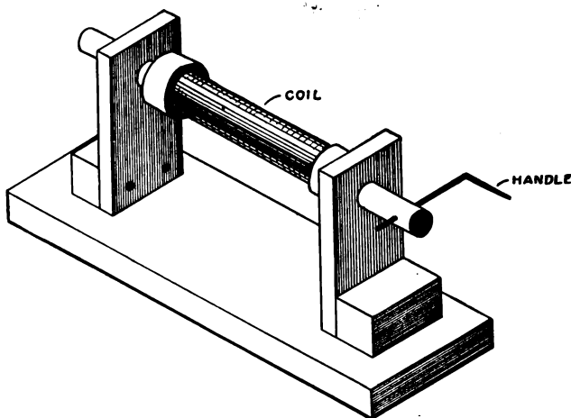
FIG. 162. — Simple Winding Device for winding the Secondary.
