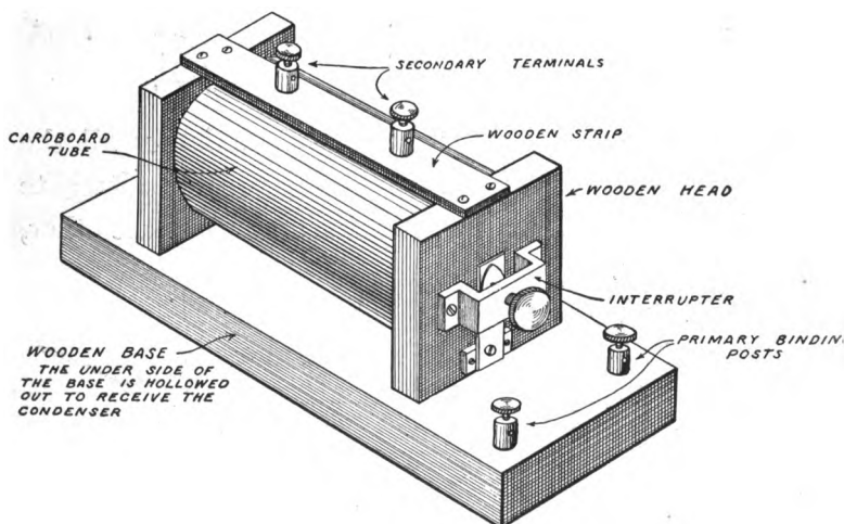
FIG. 166. — Completed Coil.
