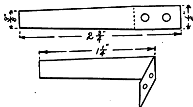
FIG. 261. — The Brushes.
