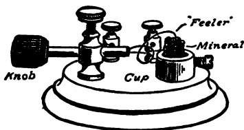
FIG. 213. — Another Form of the "Cat-Whisker" Detector.
