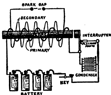
FIG. 157. — Diagram showing Essential Parts of Induction Coil.
