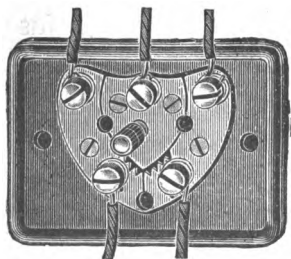
FIG. 99. — Lightning-Arrester and Ground-Wire Switch.
