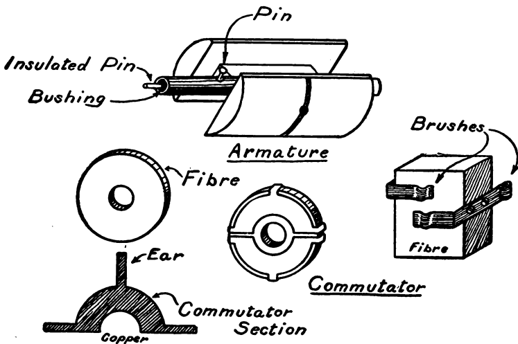
FIG. 253. — Details of the Armature, Commutator, and Brushes.
