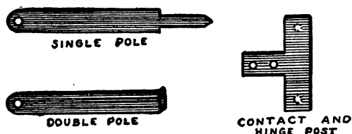
FIG. 97. — Metal Parts for the Knife Switches.
