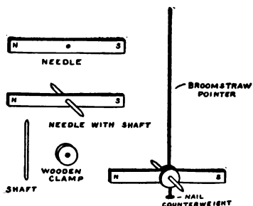
FIG. 103. — Arrangement of the Needle and Pointer.
