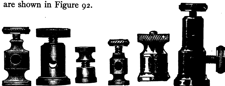
FIG. 92. — Types of Binding-Posts.
