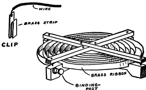
FIG. 226. — A Helix and Clip.
