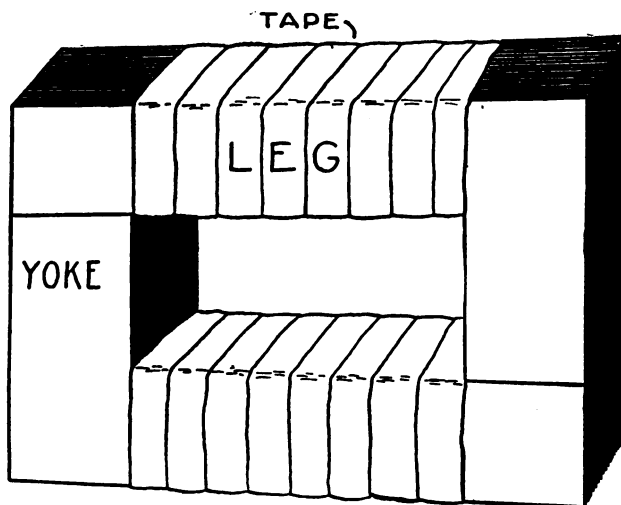
FIG. 181. — The Core, Assembled and Taped.
