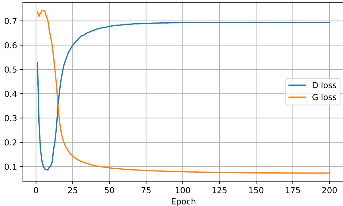
Training Loss (v10_cross split70)
