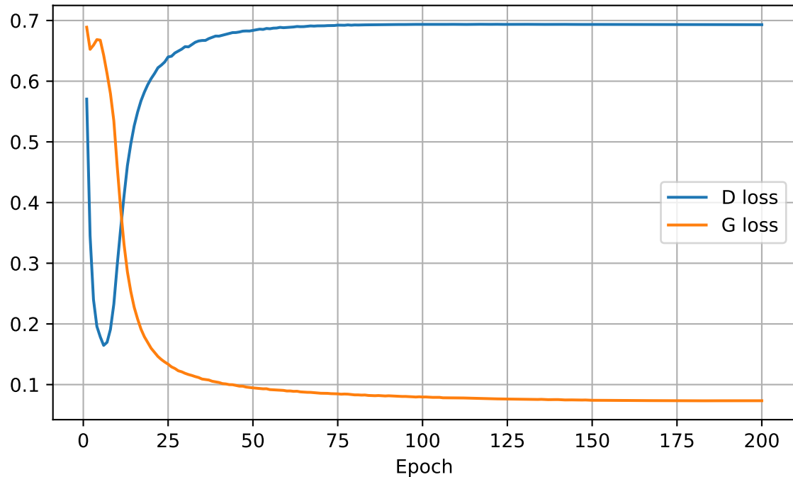
Training Loss (v10_cross split80)
