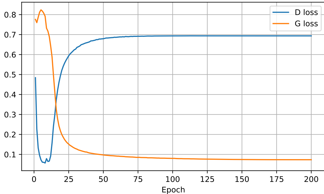
Training Loss (v10_new)
