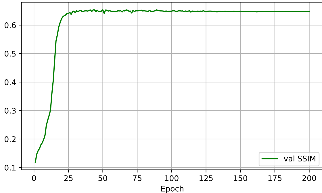
Validation SSIM (v10_new)
