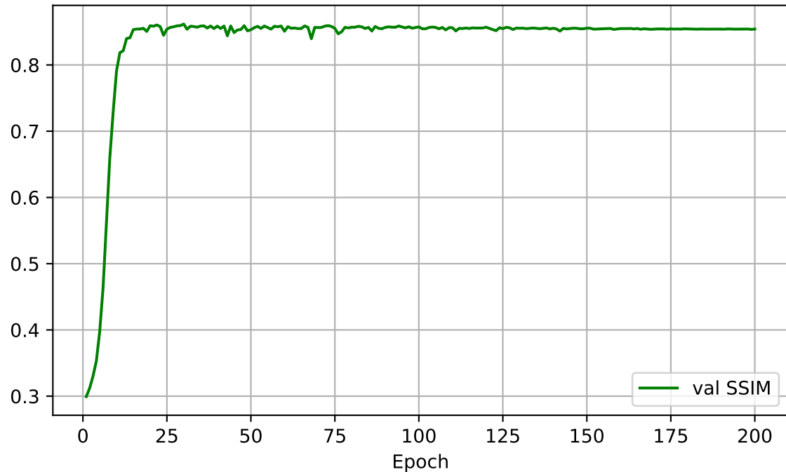
Validation SSIM
