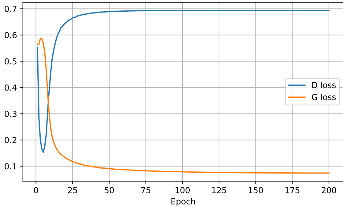
Training Loss
