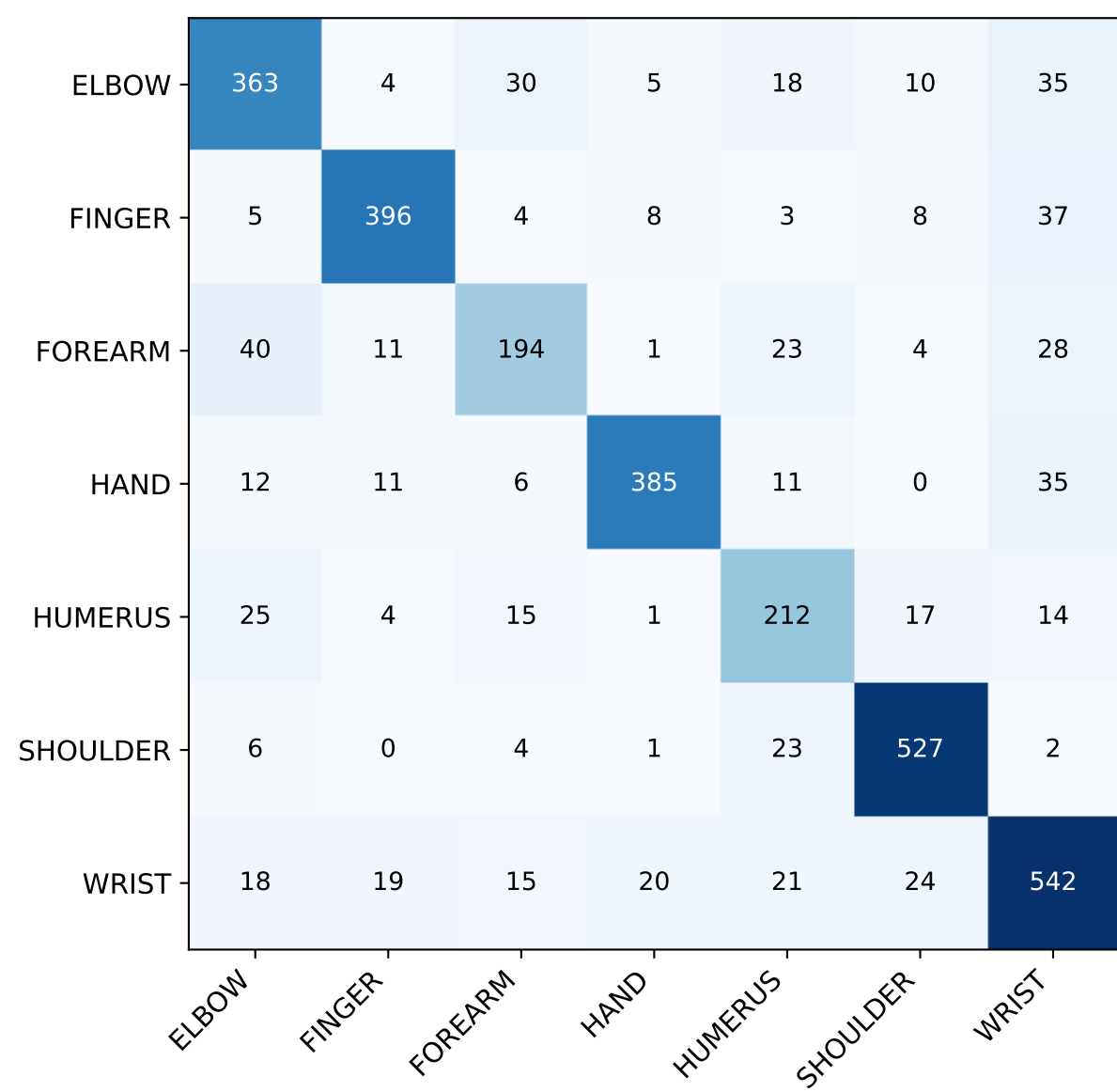
v1 ResNet — 64-ref (81.9%)
