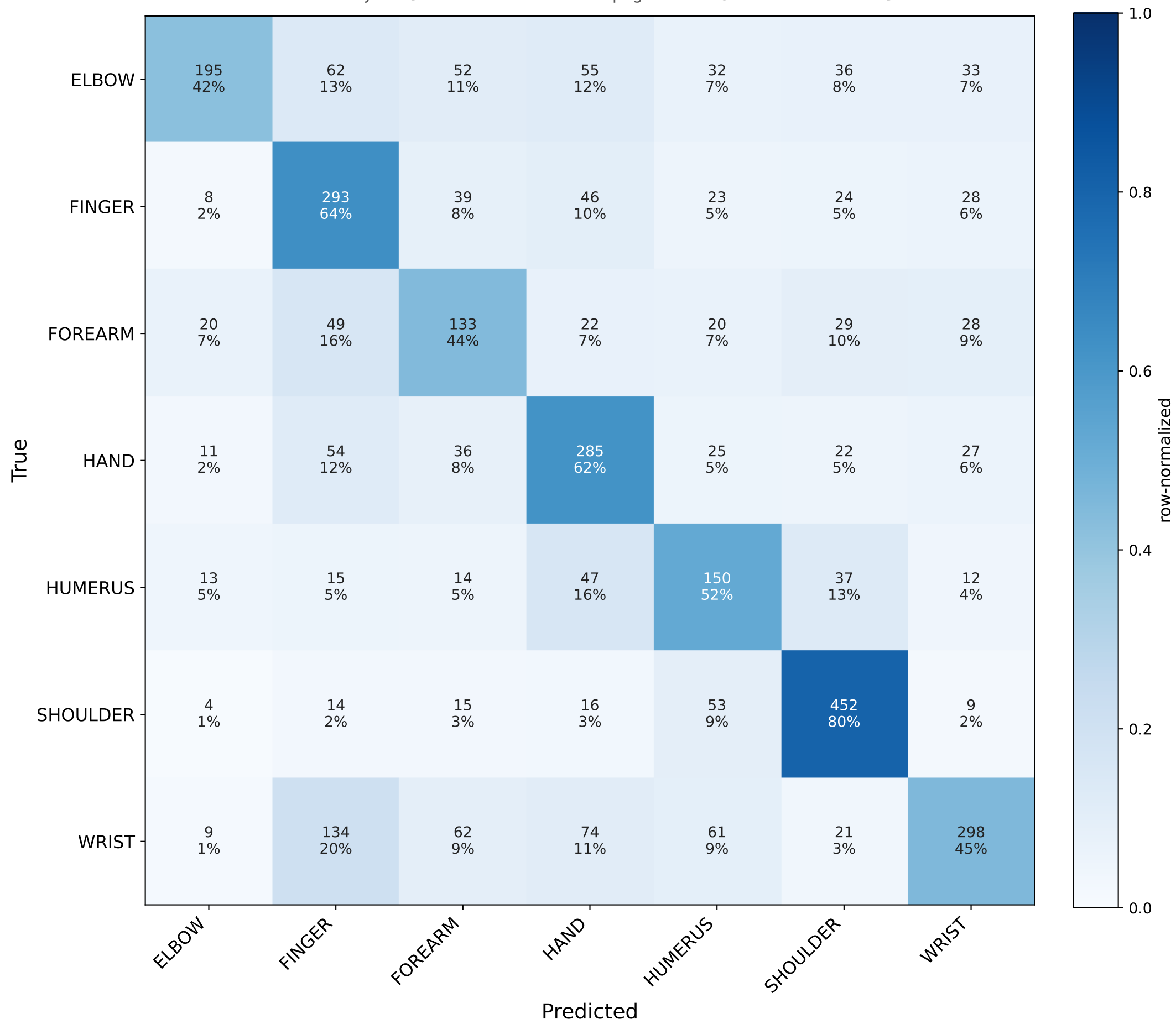
MURA body-part via write-order page reassembly
