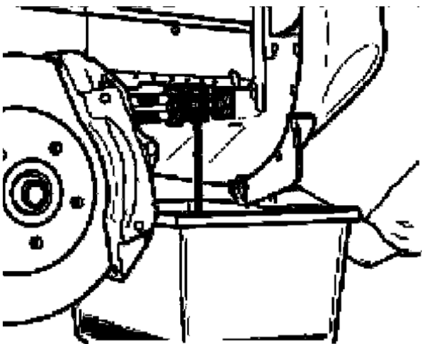
Draining cooling system
