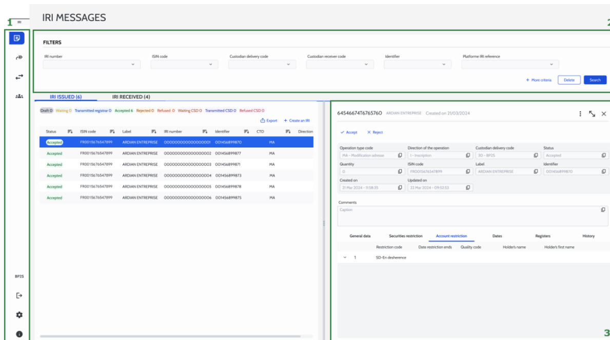
Figure 4: IRI dashboard
