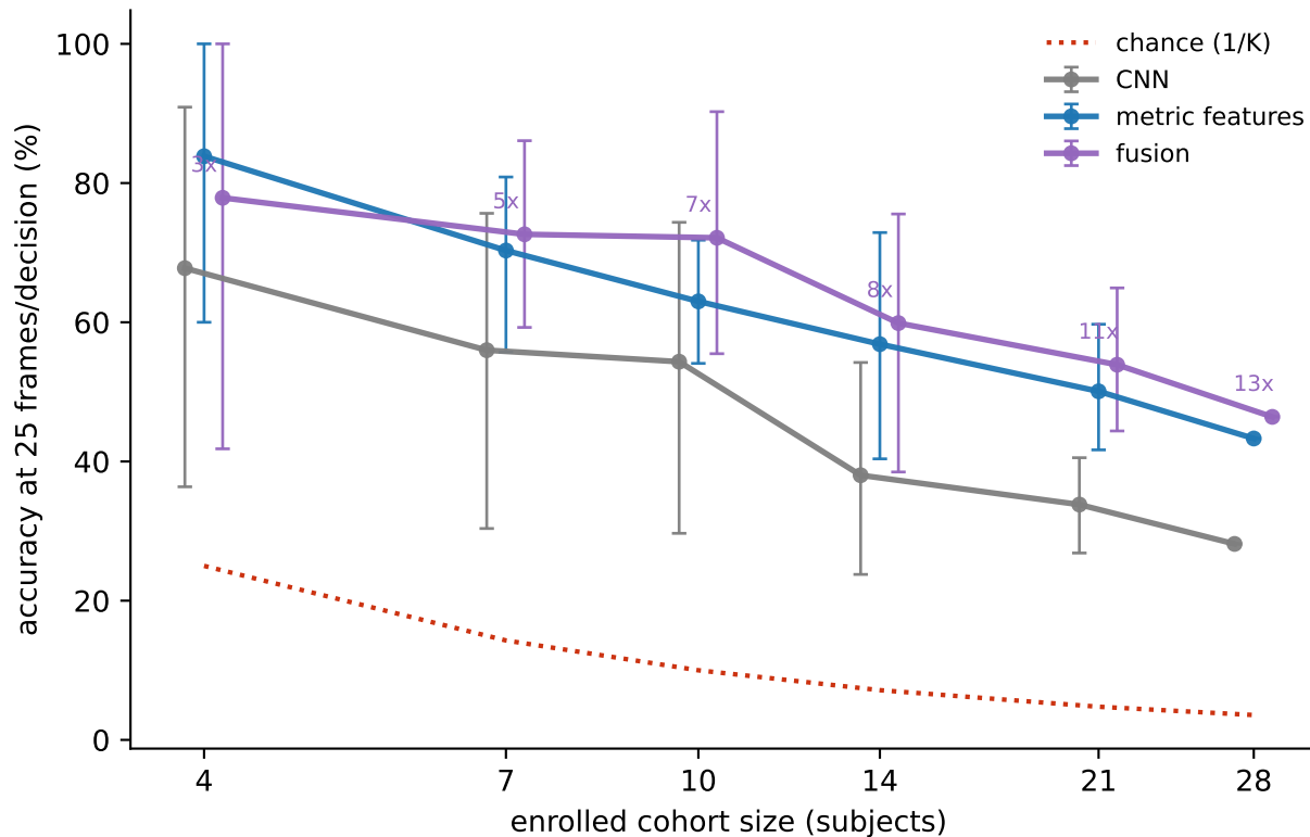
Accuracy falls with cohort size; the margin over chance grows
