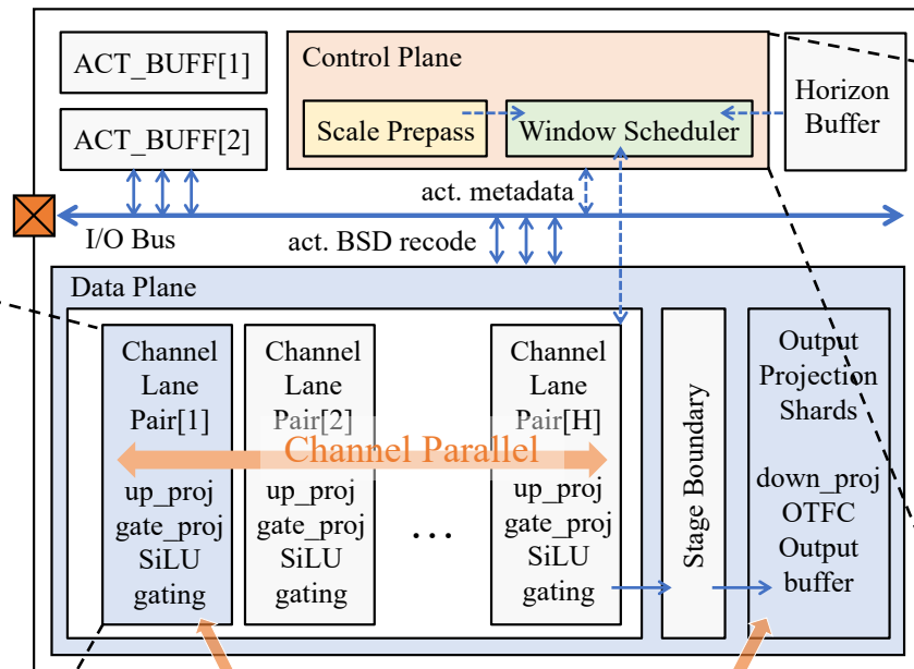
(a) Tile-level Microarchitecture
