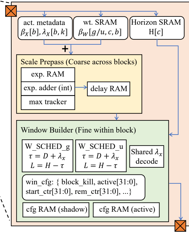
(b) Control Plane for Owner Lane Pair
