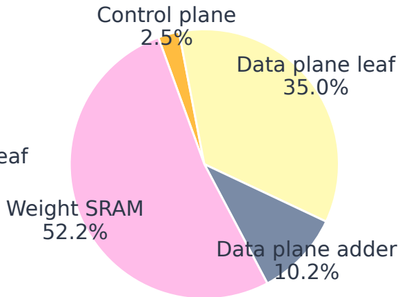
(b) Power breakdown Total Energy: 7.8\text{ mW}
