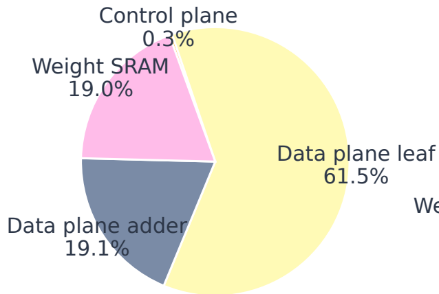
(a) Area breakdown Total Area: 0.013\text{mm}^2
