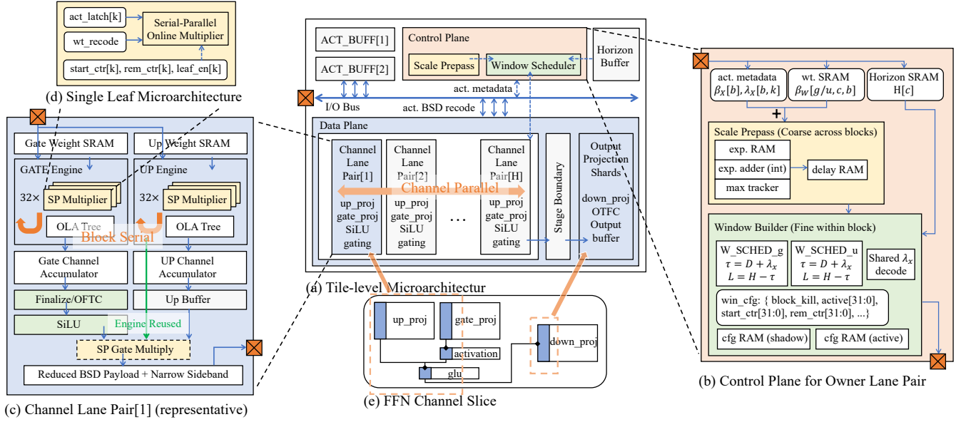
Figure 3: Channel-parallel, block-serial two-plane FFN micro-tile.
