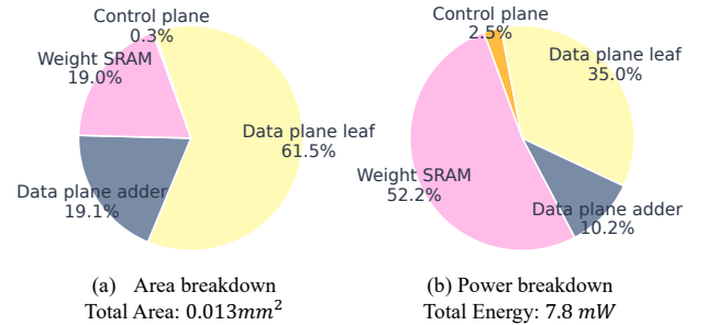
Figure 7: Per-channel area and power breakdown.
