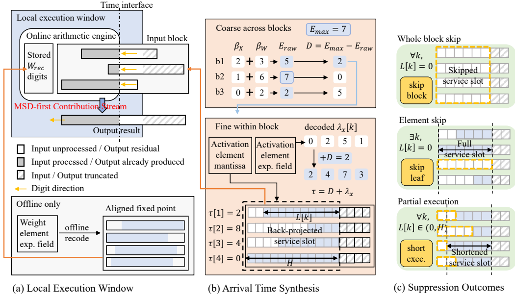
Figure 2: Local execution windows on aligned MSD-first contribution streams.
