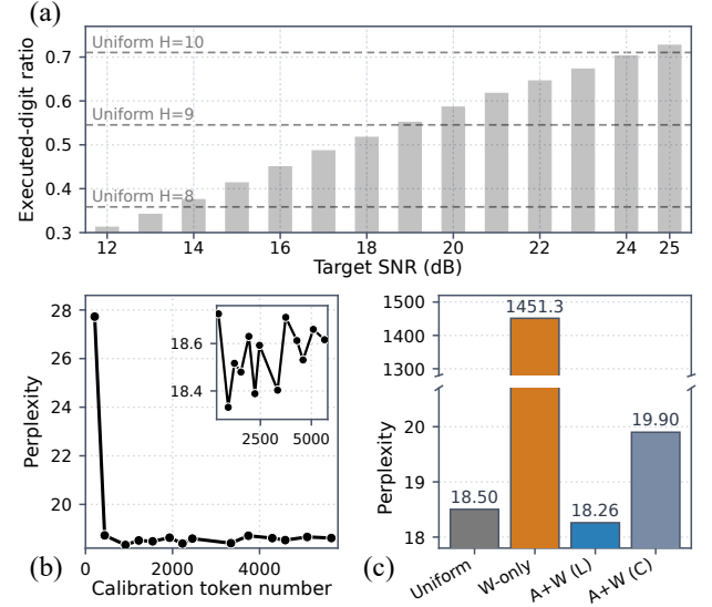
Figure 6: Validation of the offline-online split. (a) Executed-digit ratio versus initialization target SNR for layer-wise L_2 redistribution and uniform horizon. (b) Perplexity versus calibration sample size. (c) Metadata-source ablation.
