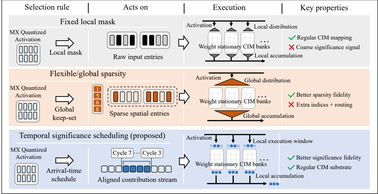
Figure 1: Temporal significance scheduling: an improved significance signal for MX-quantized CIM FFN execution.
