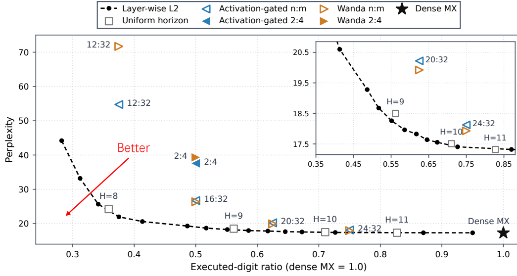
Figure 4: Quality-compute Pareto frontier for MX-quantized Qwen3-0.6B FFN inference.
