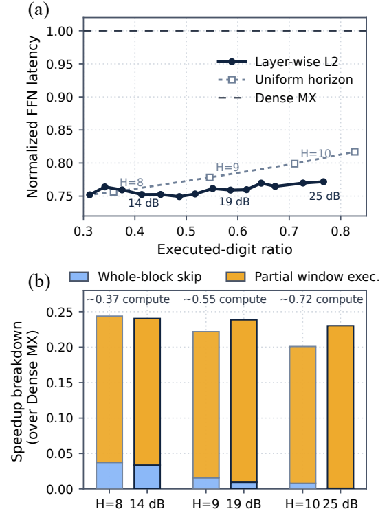
Figure 5: (a) Normalized FFN latency versus executed-digit ratio. (b) Acceleration contribution breakdown.
