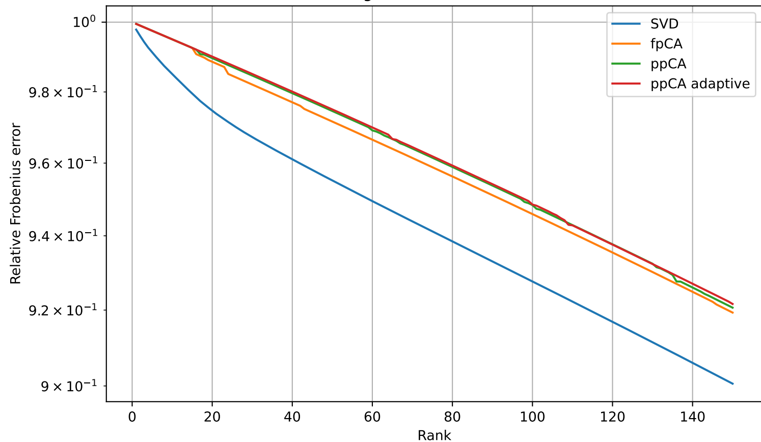
California housing Gaussian kernel matrix, n=1000
