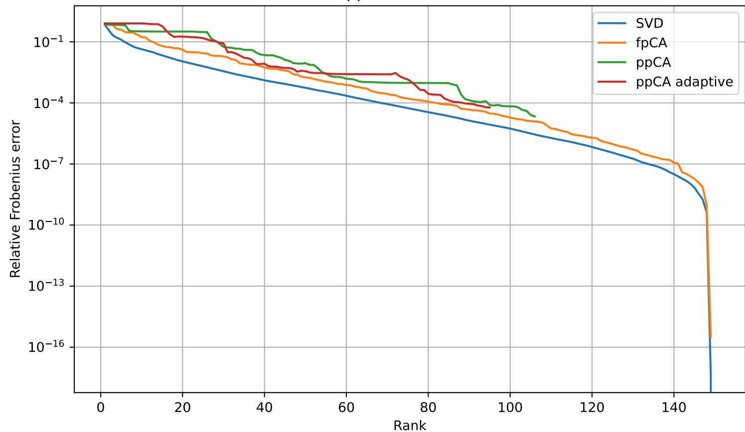
Iris kernel matrix approximation with Gaussian kernel
