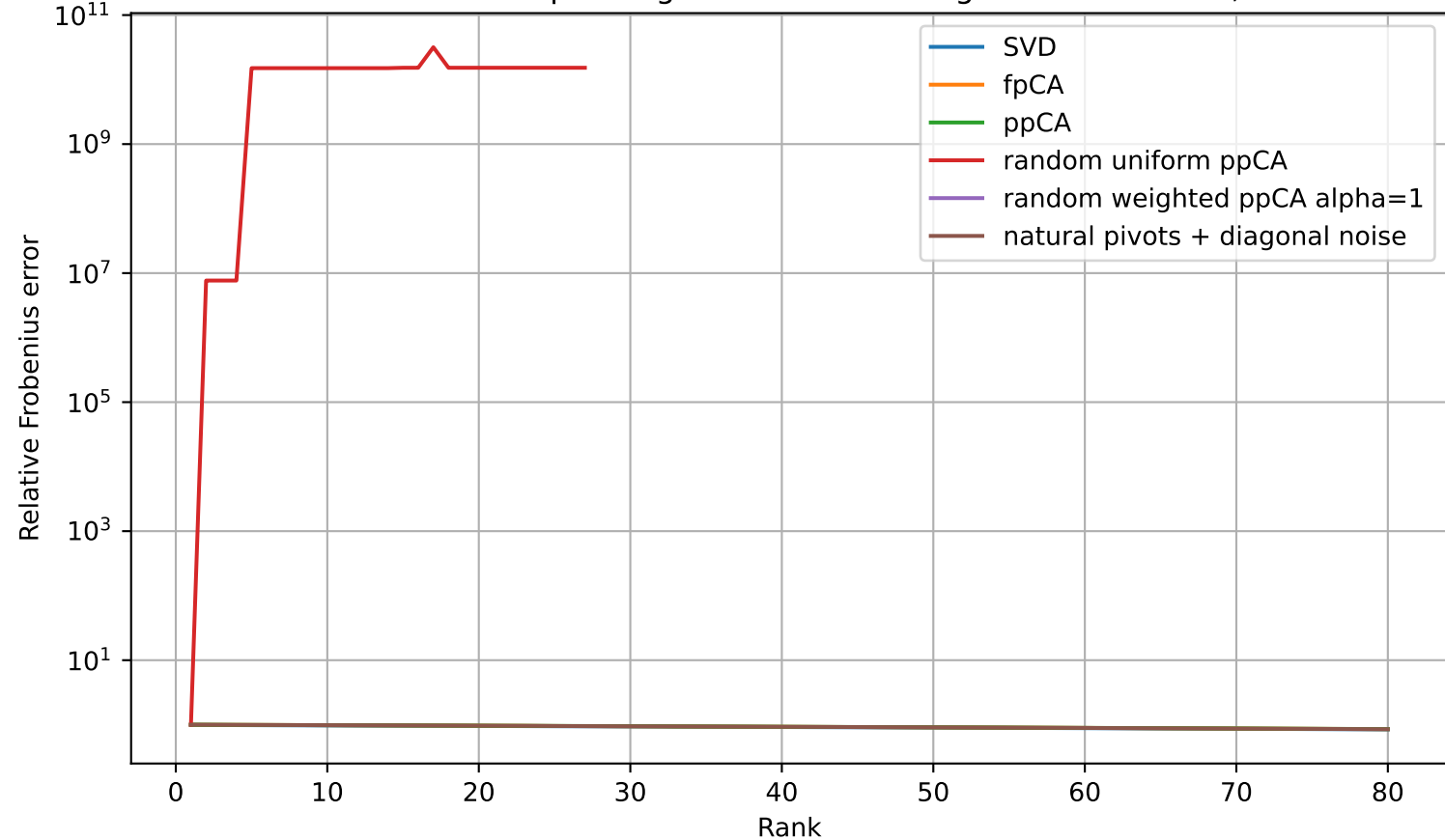
Random and natural pivoting: California housing Gaussian kernel, n=300
