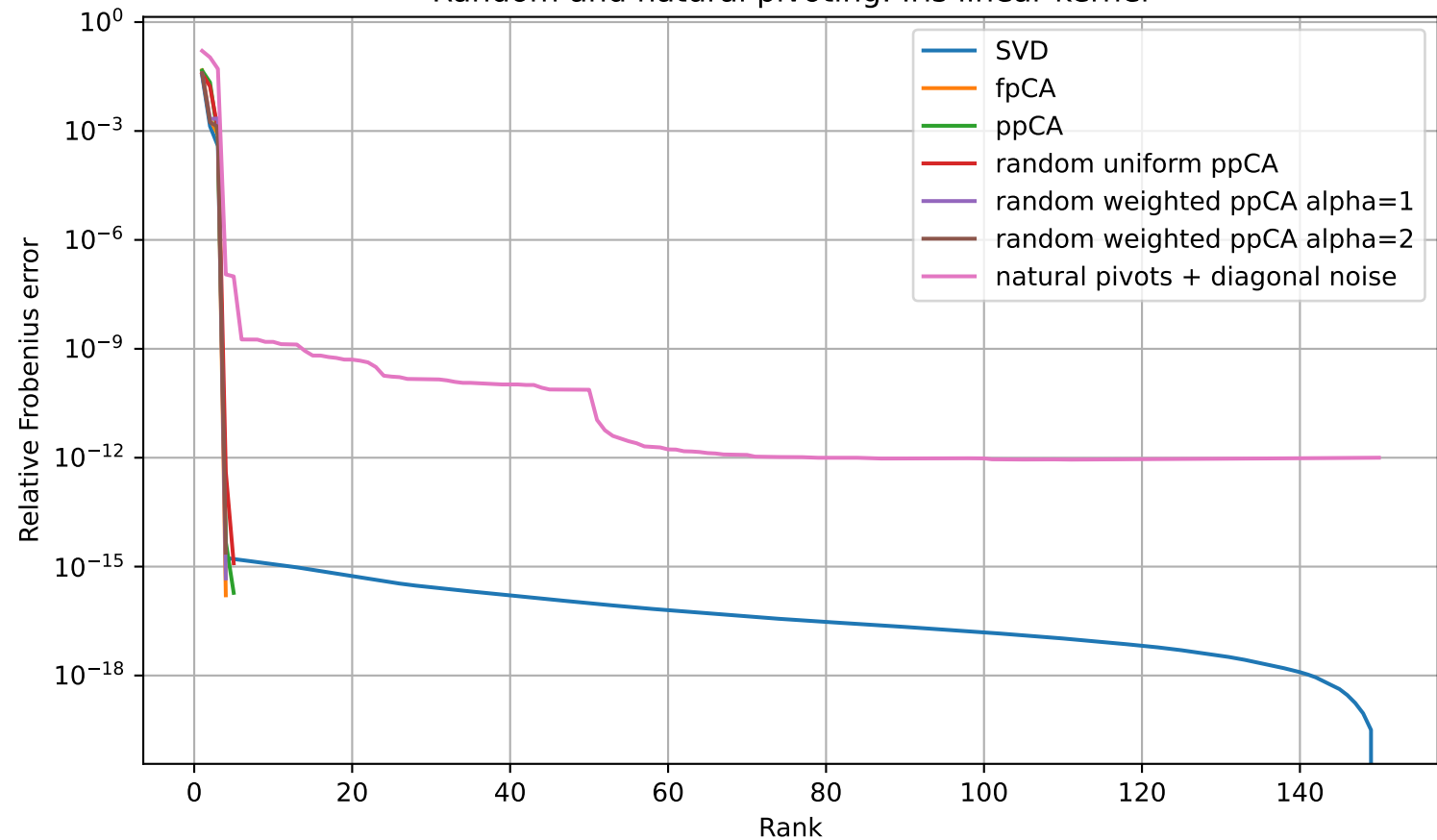
Random and natural pivoting: Iris linear kernel
