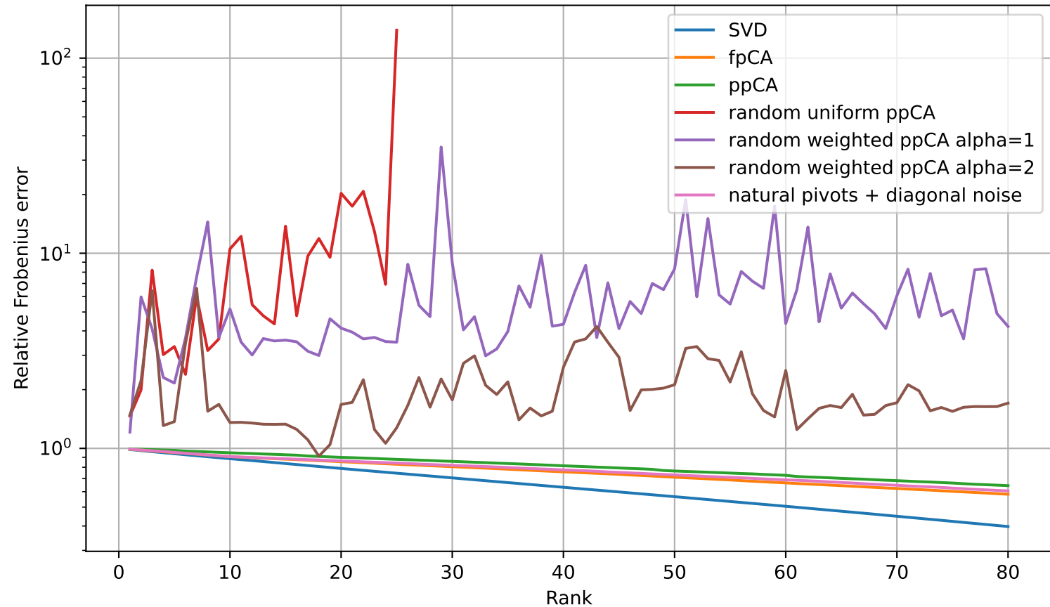
Random and natural pivoting: Synthetic A3 low-rank PSD noise
