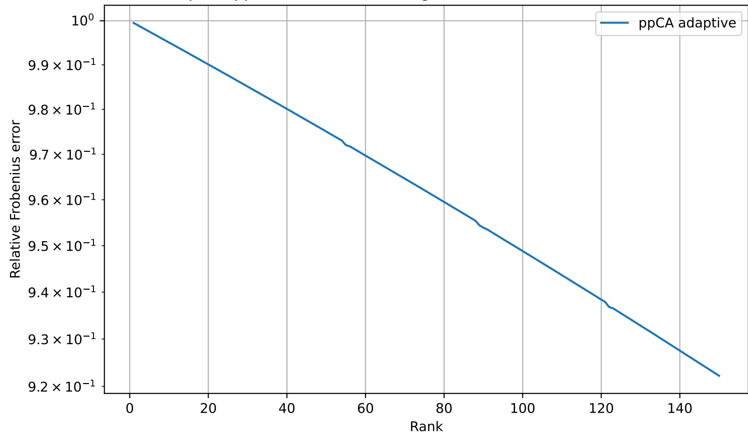
Adaptive ppCA: California housing Gaussian kernel matrix, n=1000
