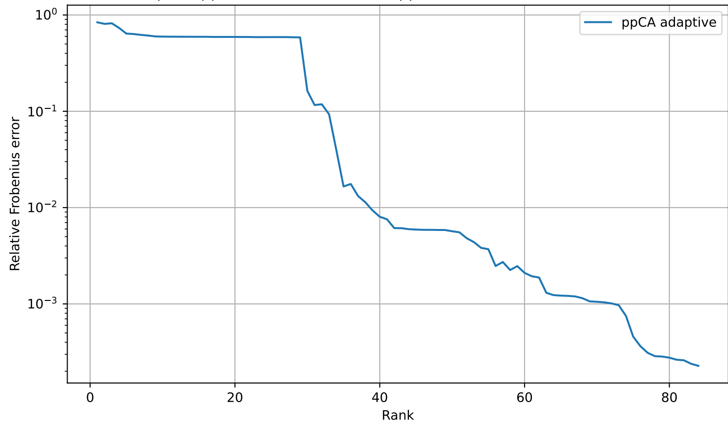
Adaptive ppCA: Iris kernel matrix approximation with Gaussian kernel
