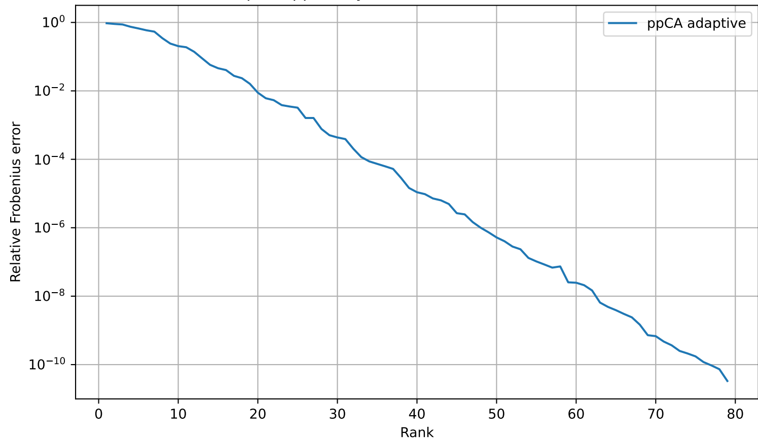
Adaptive ppCA: Synthetic test matrix A1, n=1000
