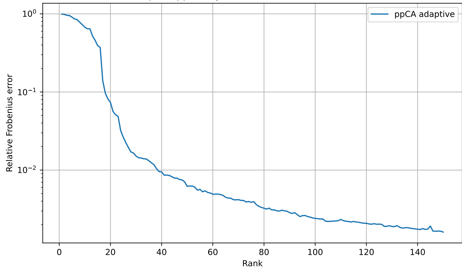
Adaptive ppCA: Synthetic test matrix A2, n=1000
