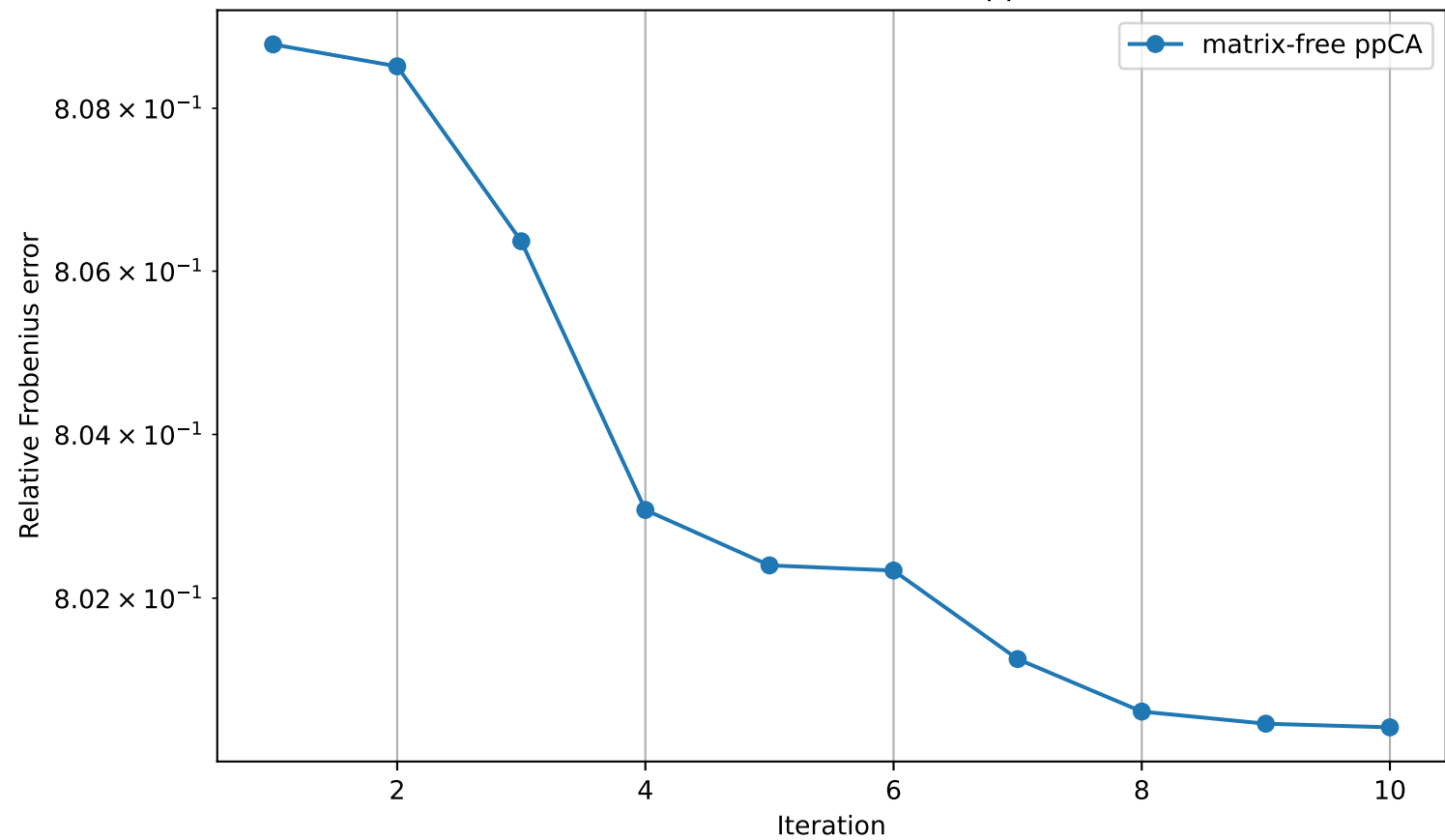
Matrix-free Iris Gaussian kernel approximation
