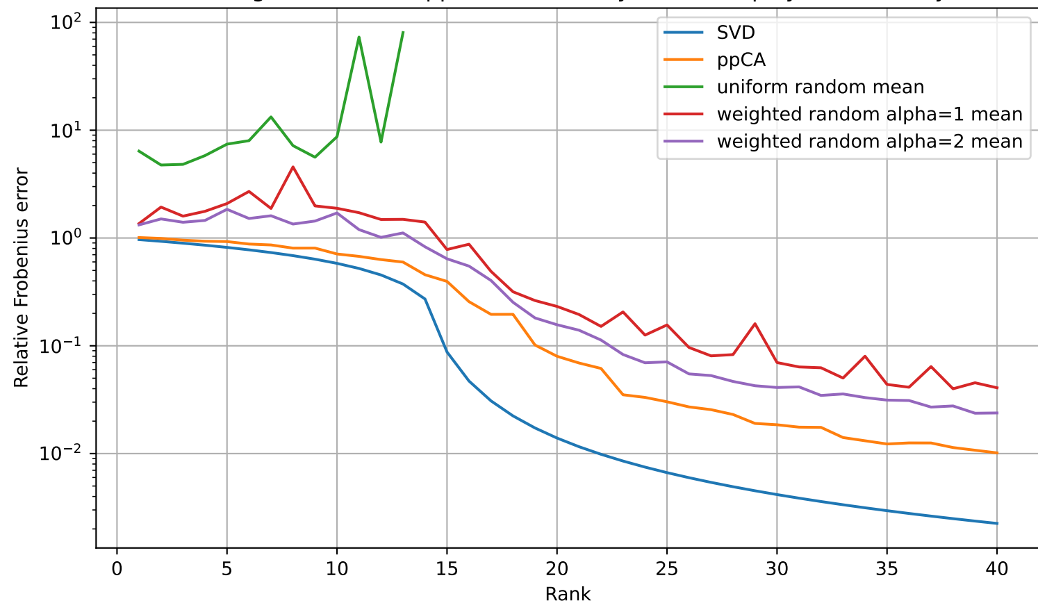
Average randomized ppCA behavior: Synthetic A2 polynomial decay
