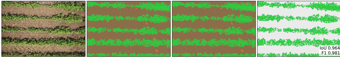
SegFormer prediction
