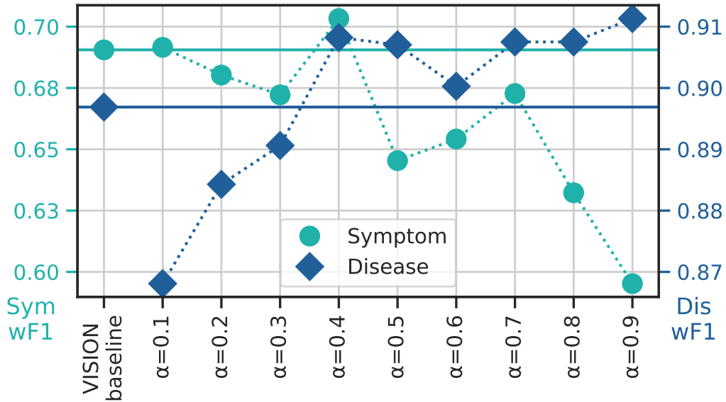
ConvNeXt MTL
