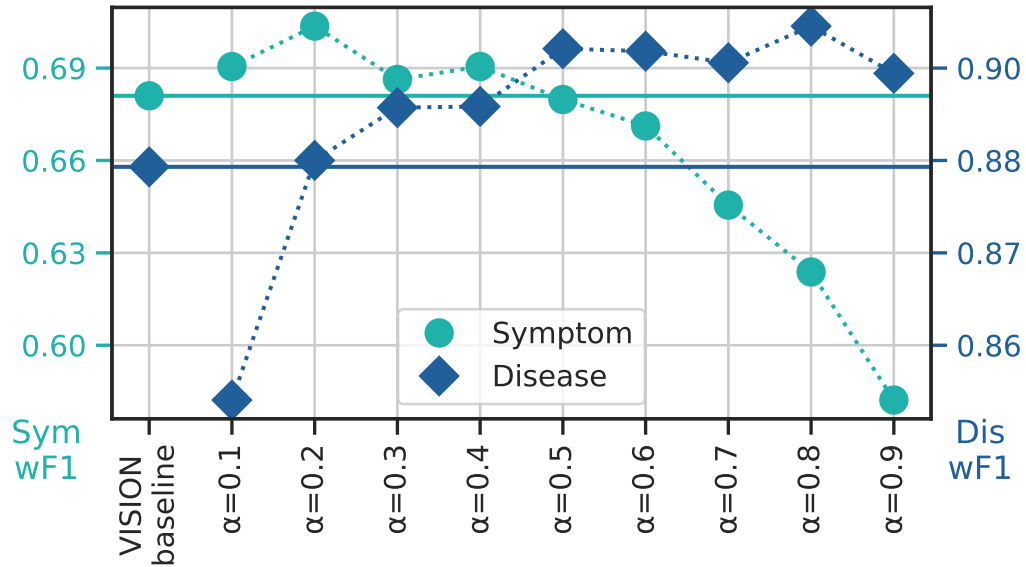
ResNet MTL
