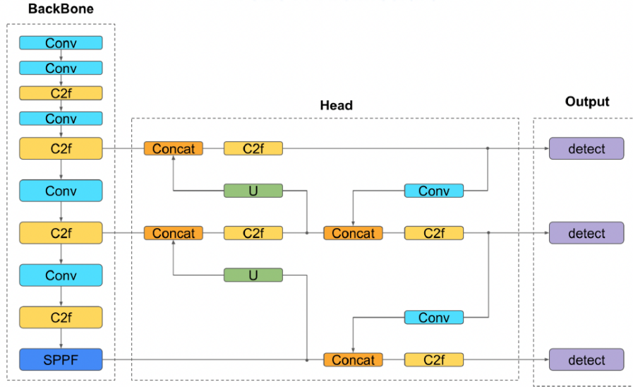
Figure 7.2: YOLOv8 architecture
